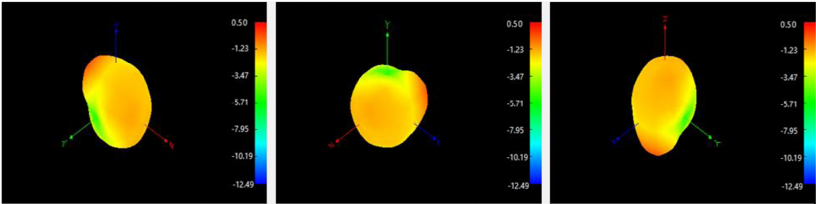
3D Radiation Pattern for 2450MHz
