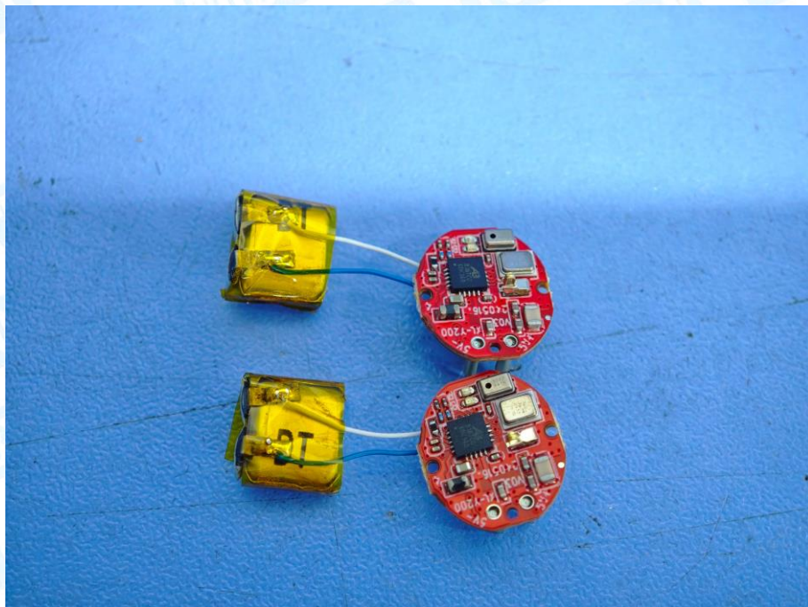
Photo 15 Appearance of PCB (Left & Right)
