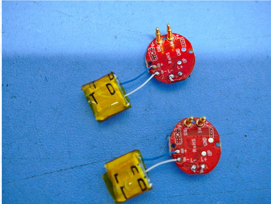
Photo 16 Appearance of PCB (Left & Right)
