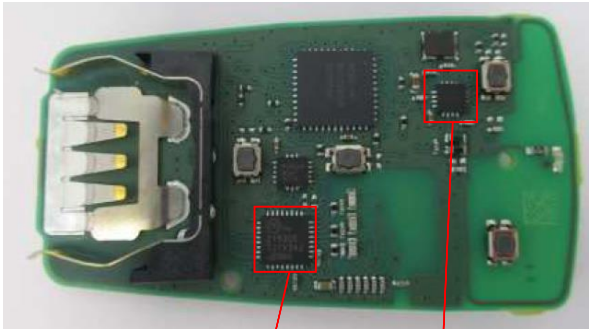
UHF Tx IC (PCF7900VHN)
