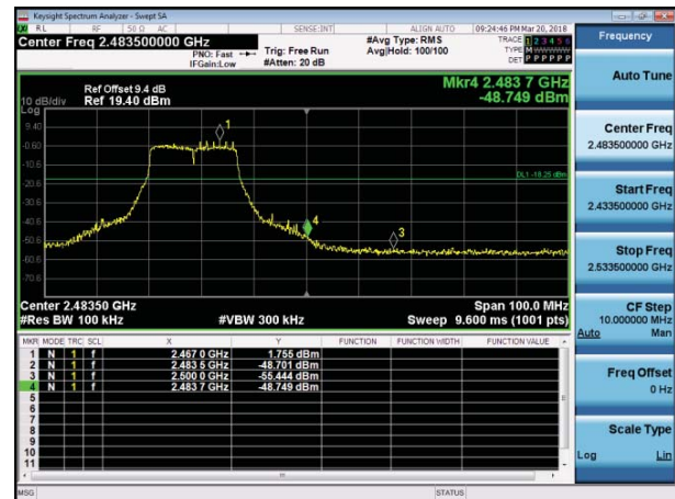
Channel 11 / 2462 MHz
