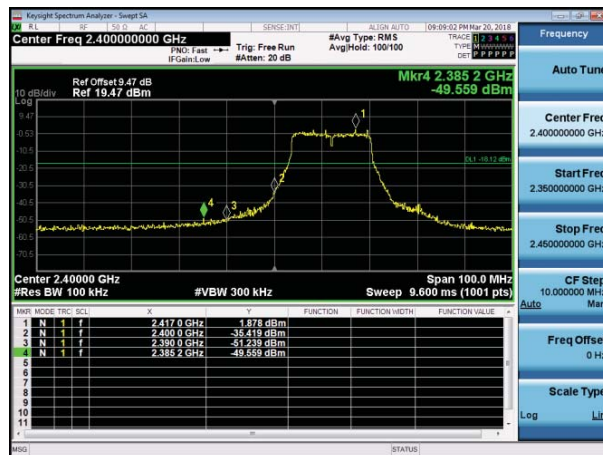
Channel 1 / 2412 MHz
