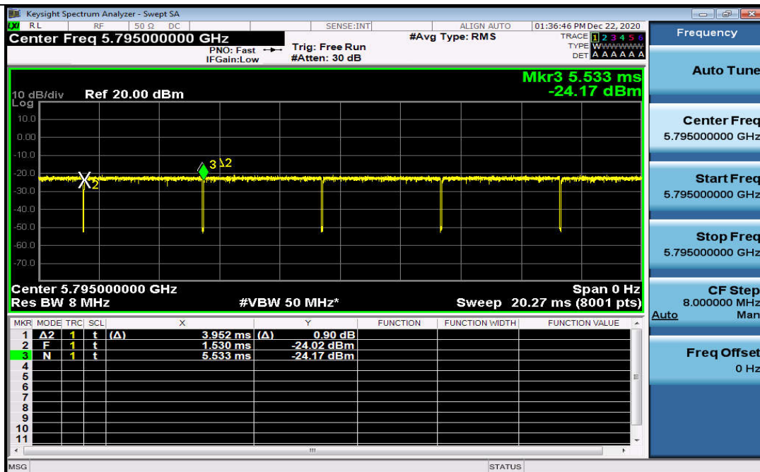
Duty Cycle_11AC40MIMO_5795_Ant2
