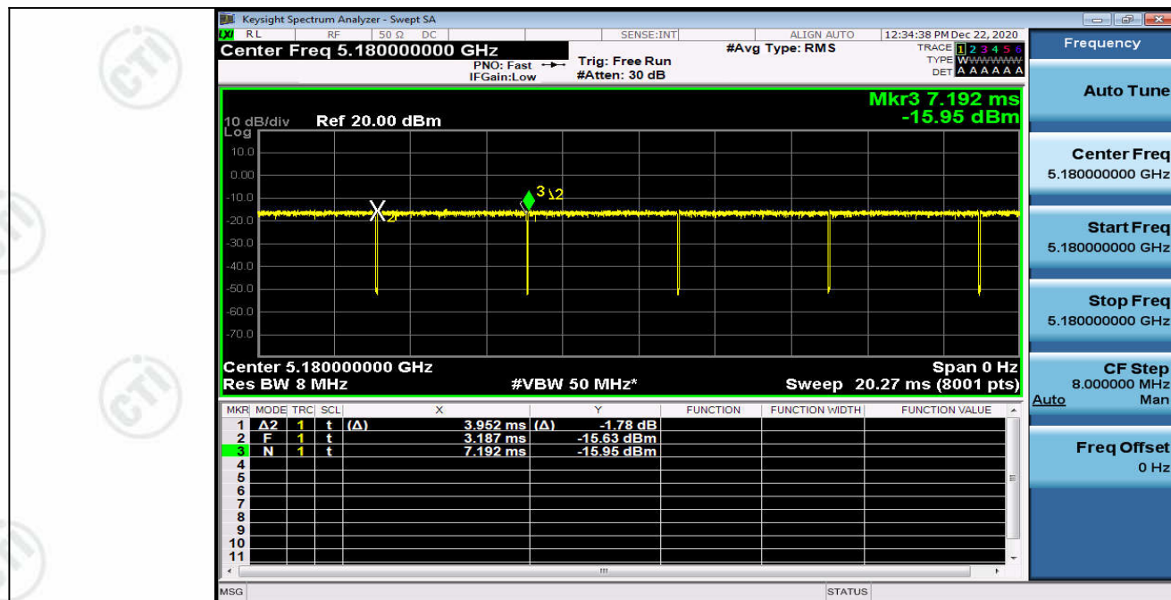
Duty Cycle_11AC20MIMO_5180_Ant2
