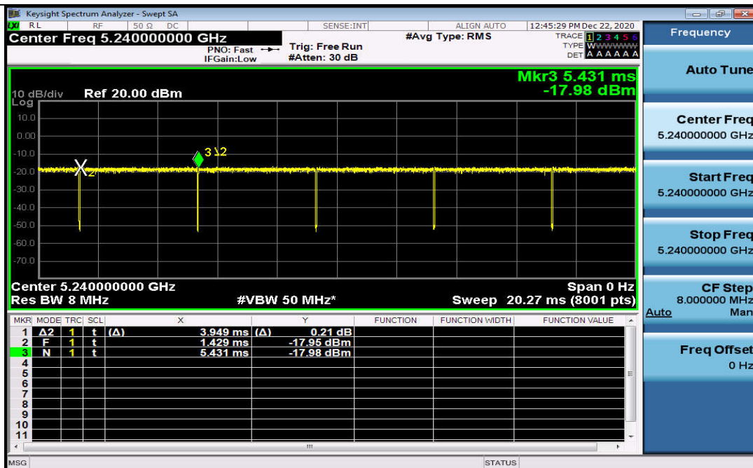
Duty Cycle_11AC20MIMO_5240_Ant2
