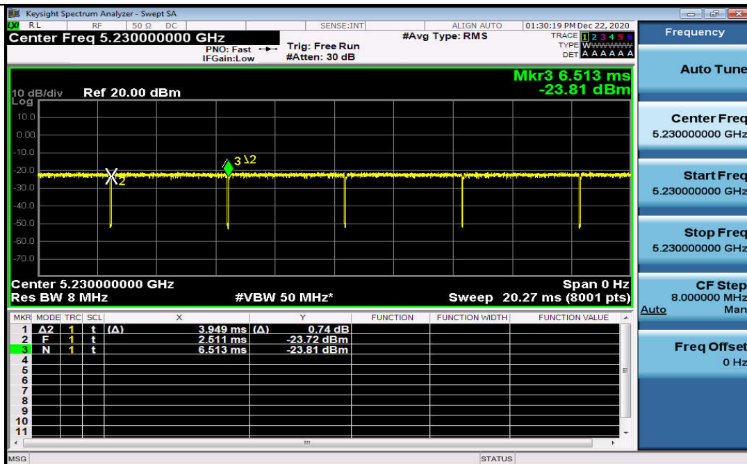
Duty Cycle_11AC40MIMO_5230_Ant2
