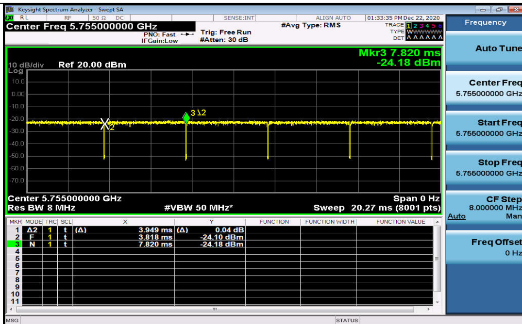
Duty Cycle_11AC40MIMO_5755_Ant2
