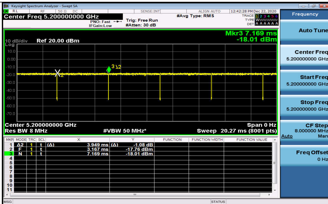
Duty Cycle_11AC20MIMO_5200_Ant2
