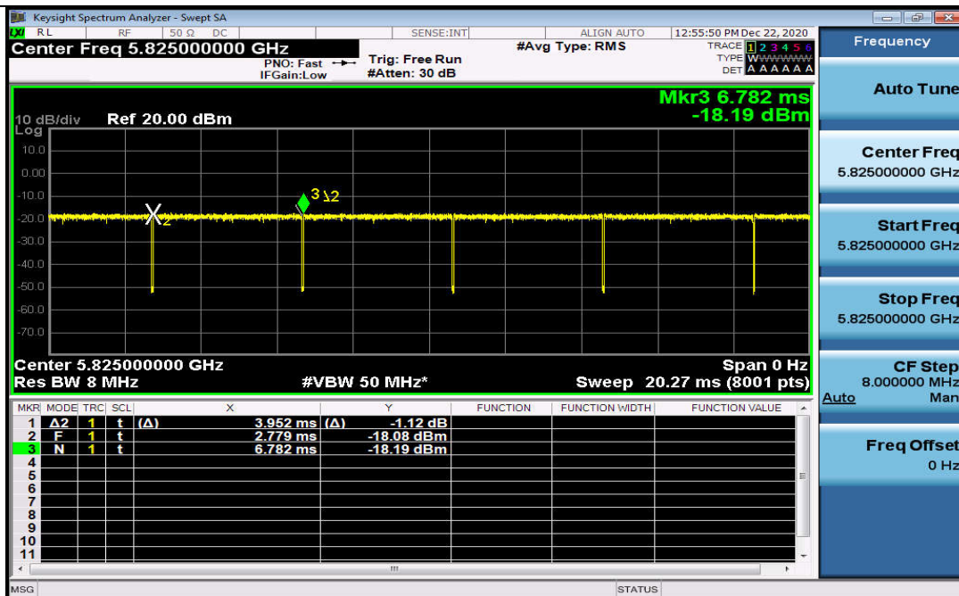
Duty Cycle_11AC20MIMO_5825_Ant2
