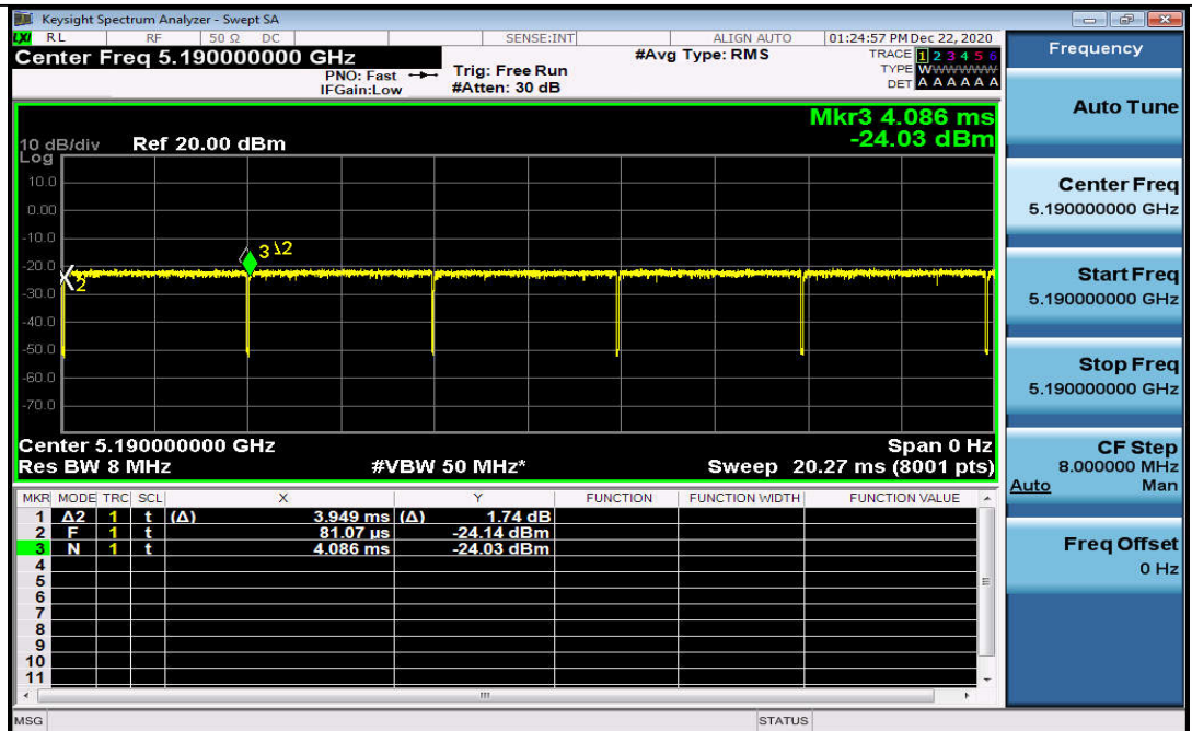
Duty Cycle_11AC40MIMO_5190_Ant2
