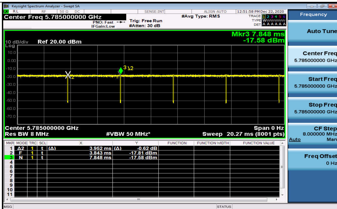
Duty Cycle_11AC20MIMO_5785_Ant2
