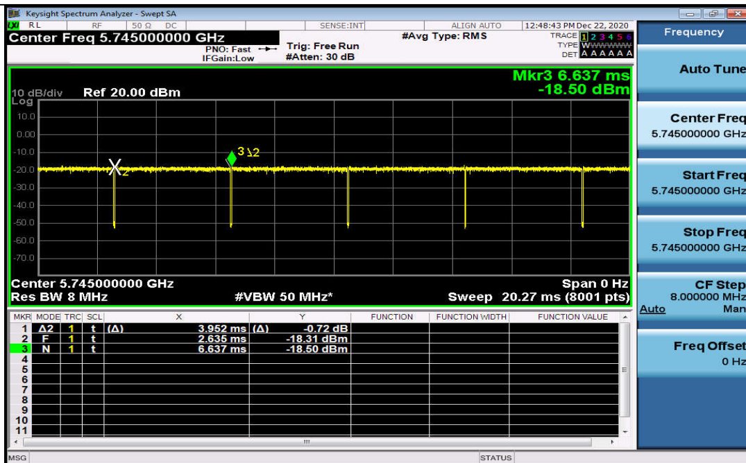
Duty Cycle_11AC20MIMO_5745_Ant2
