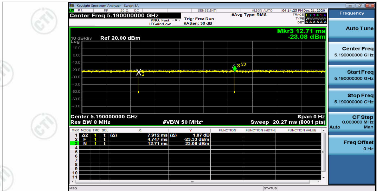
Duty Cycle_11N40MIMO_5230_Ant2
