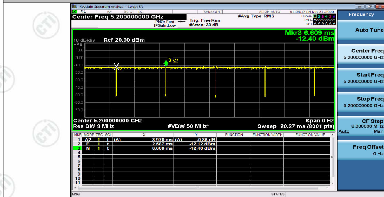
Duty Cycle_11N20_5240_Ant1
