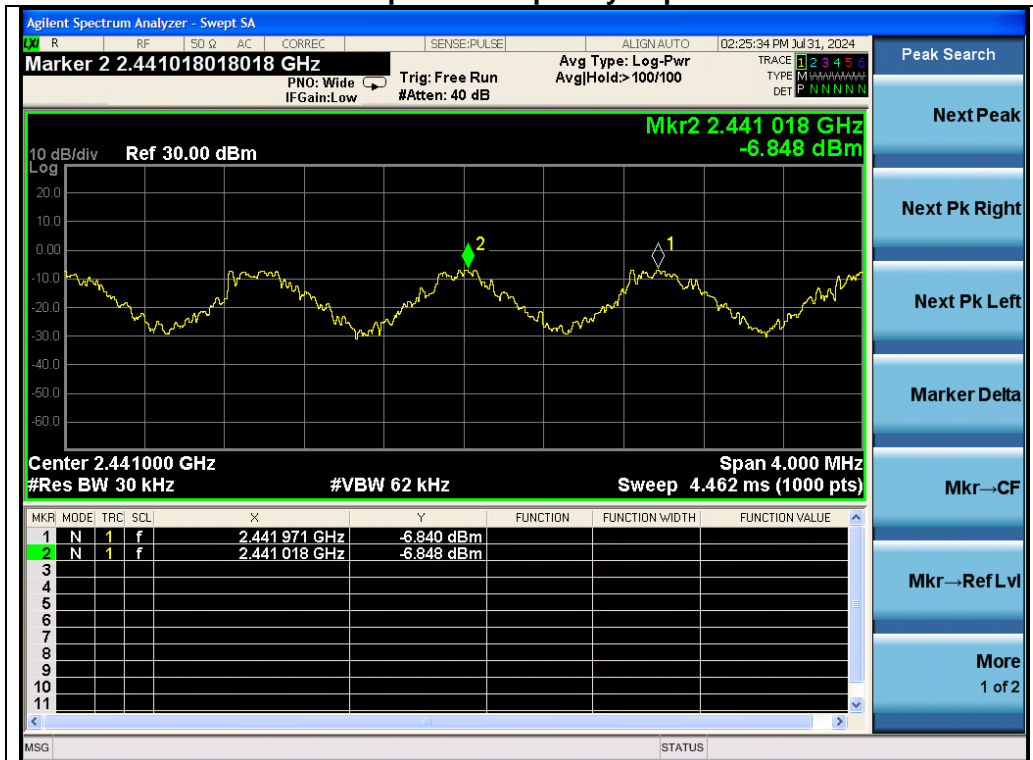
Test_Graph_BR_HOP_ANT1_NA_1Mbps_Hopping Separation
