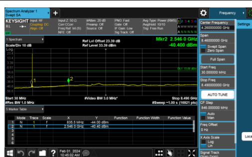
B5-1.4M-Low CH-CSE-1-QPSK-1 RB 0
