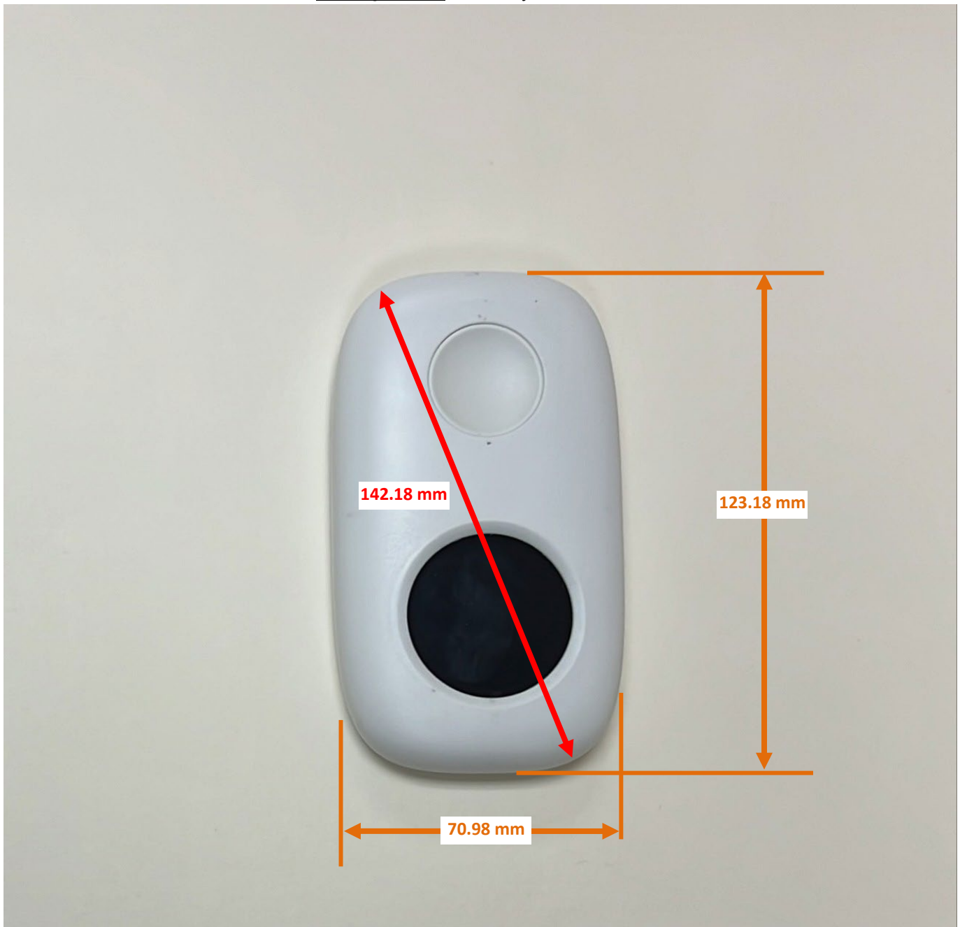
Photograph 1: Gateway Dimensions
