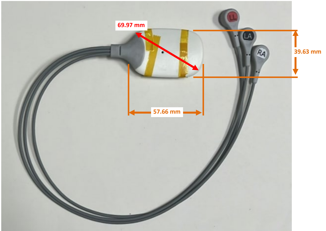
Photograph 2: Sensor Dimensions
