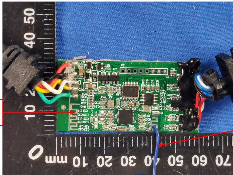
Bluetooth Antenna
