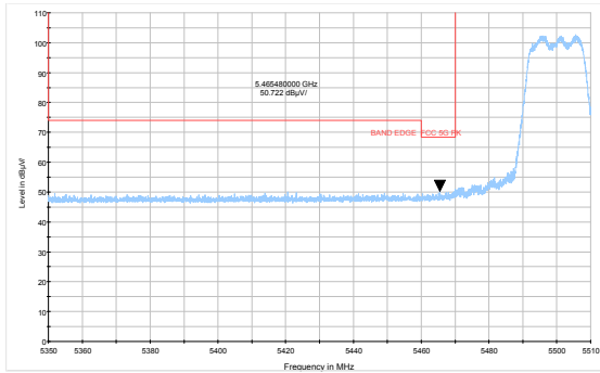
802.11a-Channel 100: Average
