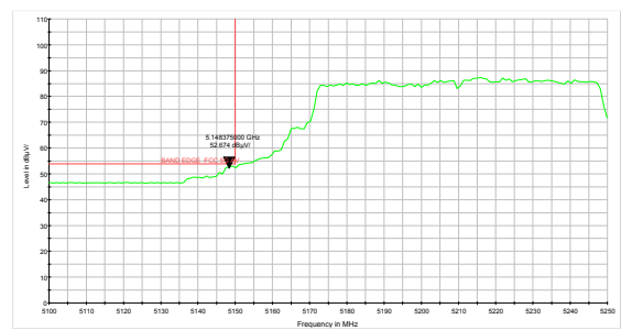
802.11ac VHT80- Channel 42: Average
