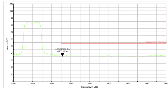
802.11a-Channel 64: Average
