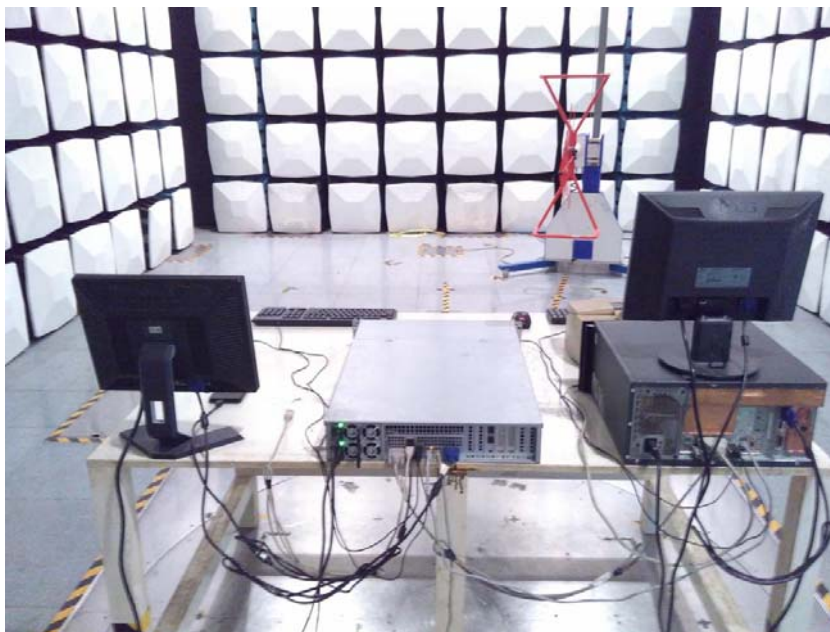
Radiated Emissions Test Setup - Rear View (Below 1GHz)
