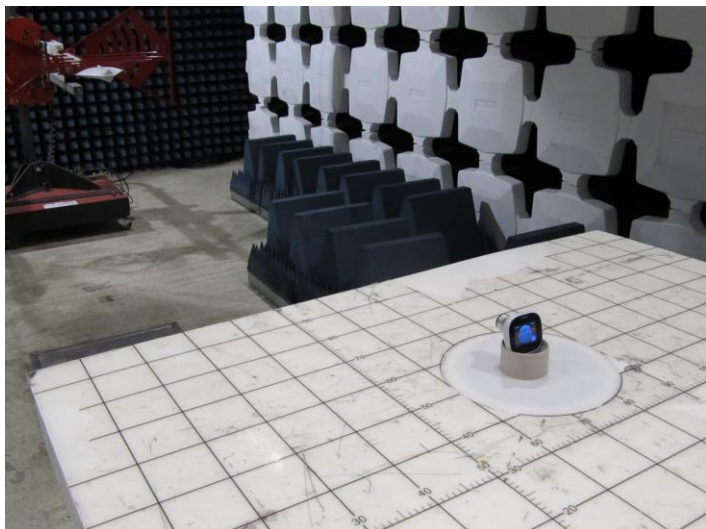
Photo 1. Radiated Emission 30MHz-1GHz
