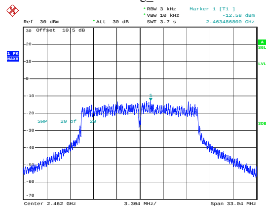
802.11g_2462MHz
