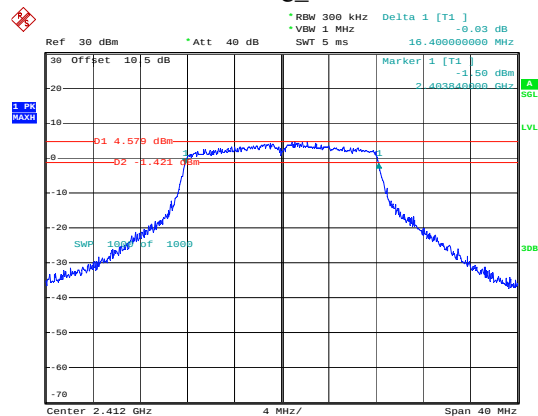
802.11g_2412MHz
