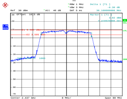
802.11n40_2437MHz
