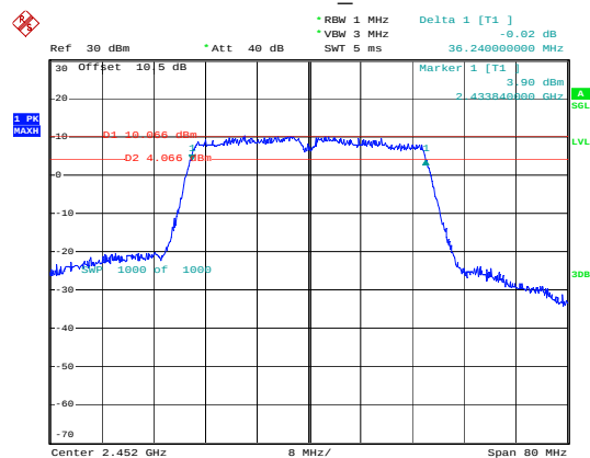
802.11n40_2452MHz
