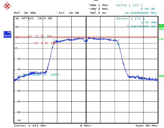
802.11n40_2422MHz
