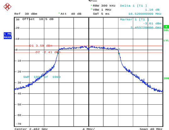
802.11g_2462MHz
