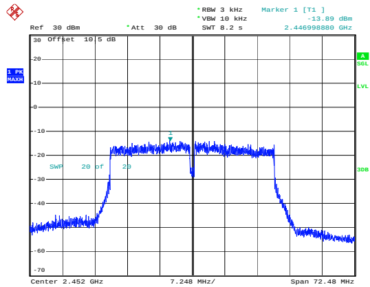
802.11n40_2452MHz
