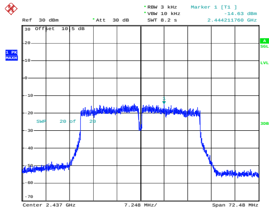
802.11n40_2437MHz
