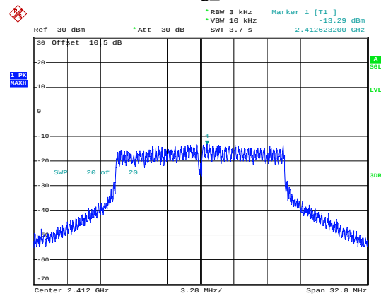
802.11g_2412MHz
