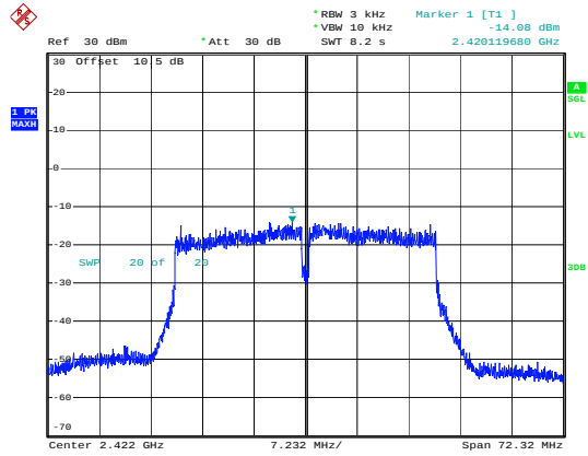
802.11n40_2422MHz
