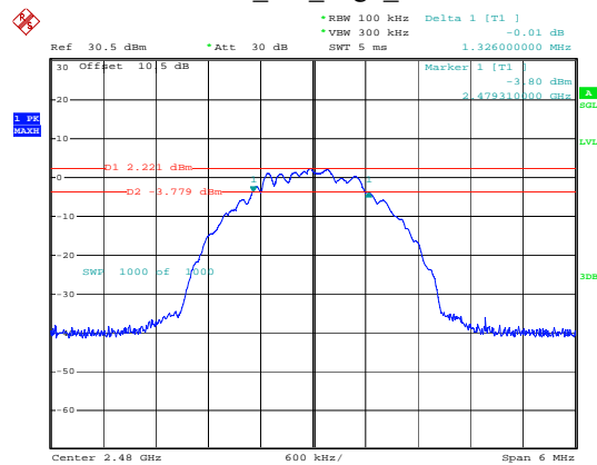
BLE_2M_High_Channel
