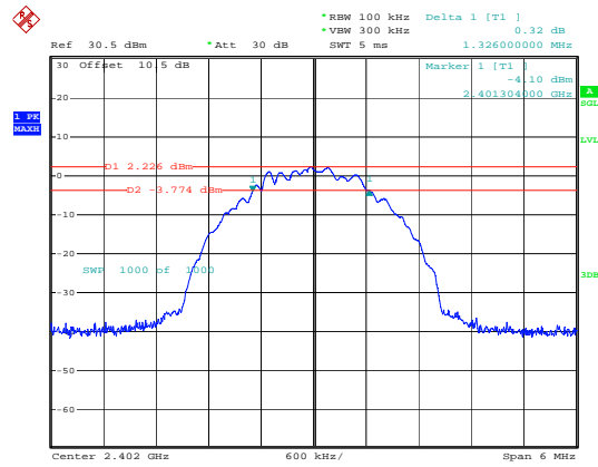
BLE_2M_Low_Channel
