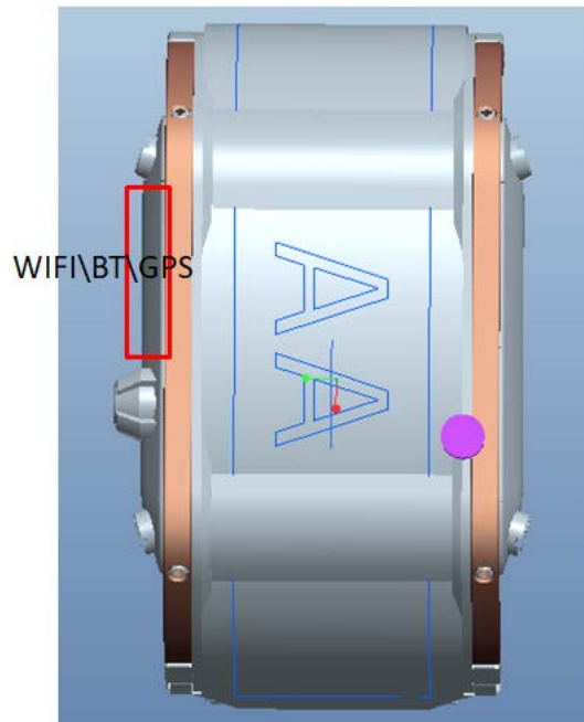
Fig.12.1 EUT Antenna Locations
