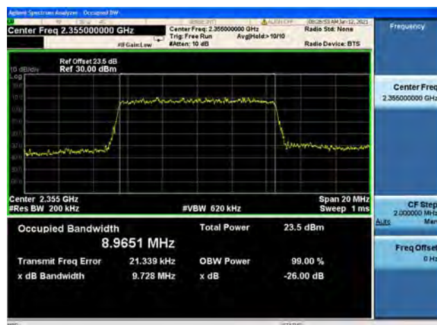
Band40/ Block B / 10MHz / Mid CH / 16QAM
