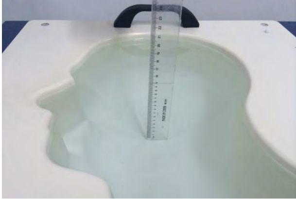
Head Liquid Depth (5GHz)
