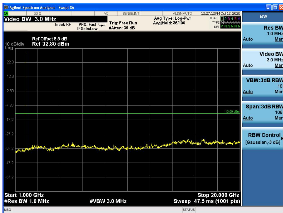
Channel 661, 1GHz~20GHz
