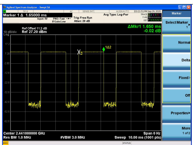
Modulation type: GFSK DH3 2441MHz
