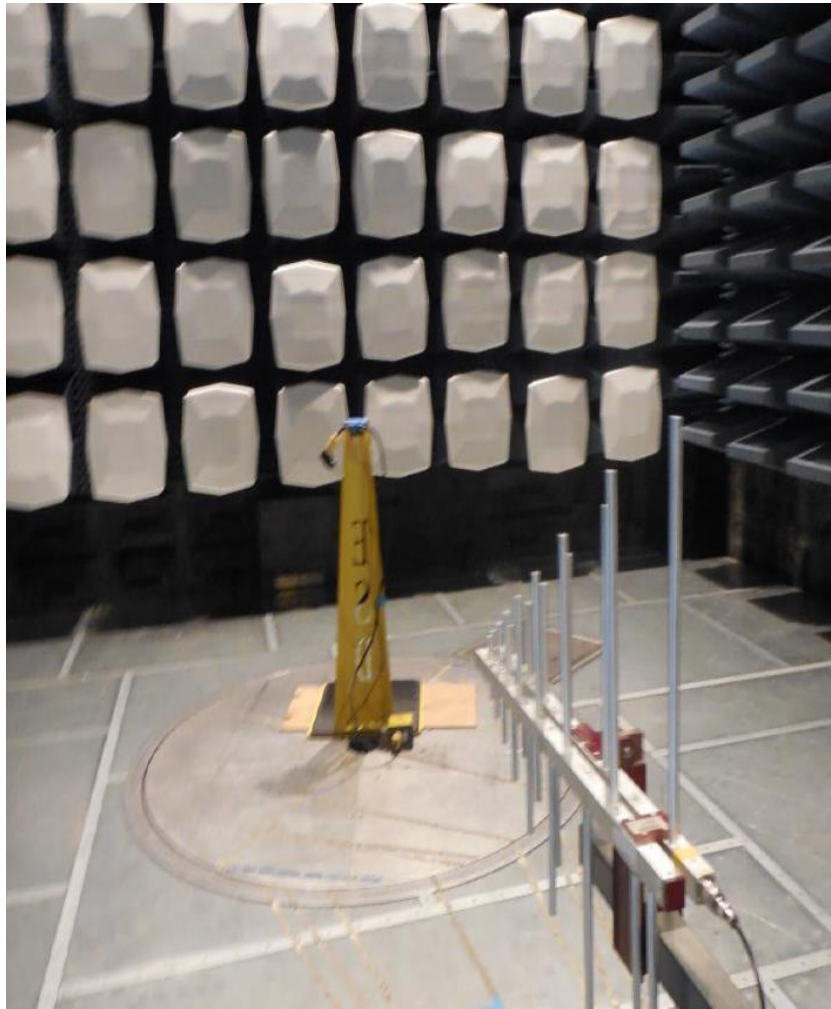
Radiated Emission Test Setup, above 200MHz
