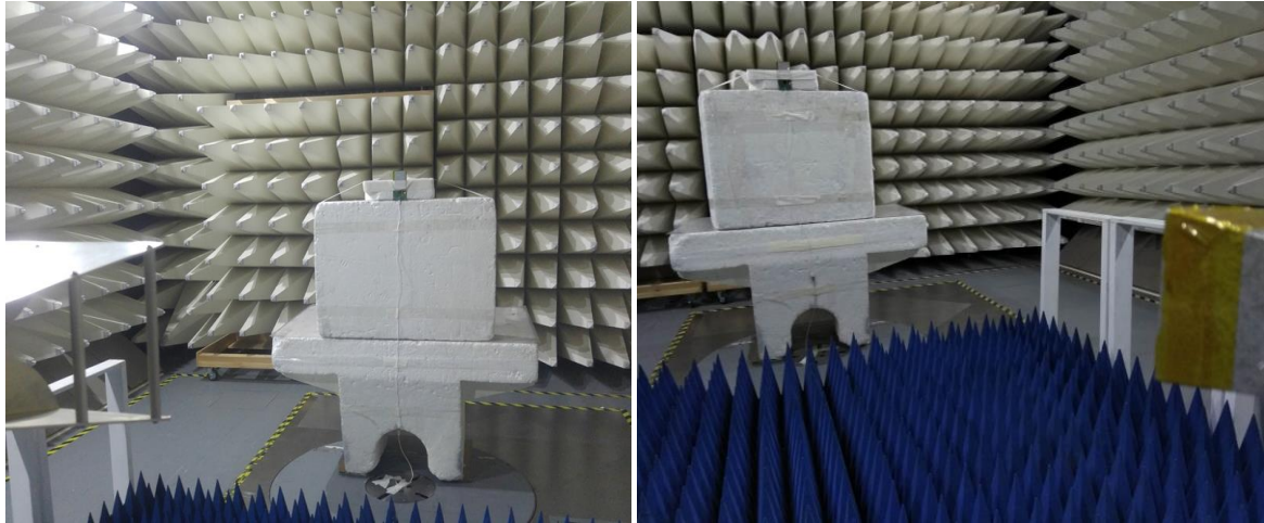
Photograph No.4 Spurious and band edge emissions measurement setup in the anechoic chamber above 1 GHz
