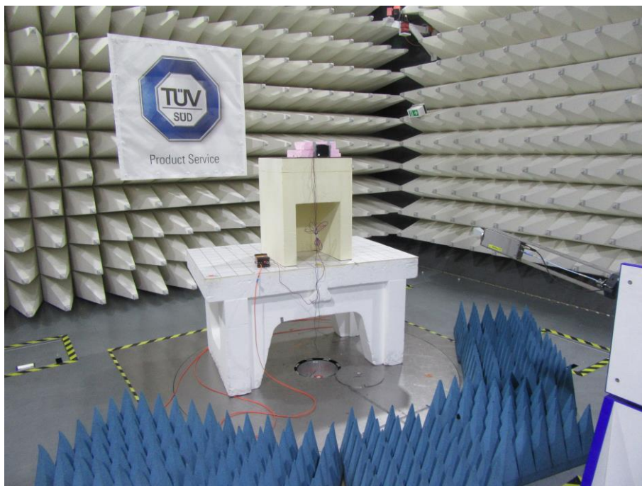
Radiated Emissions 18 – 40 GHz
