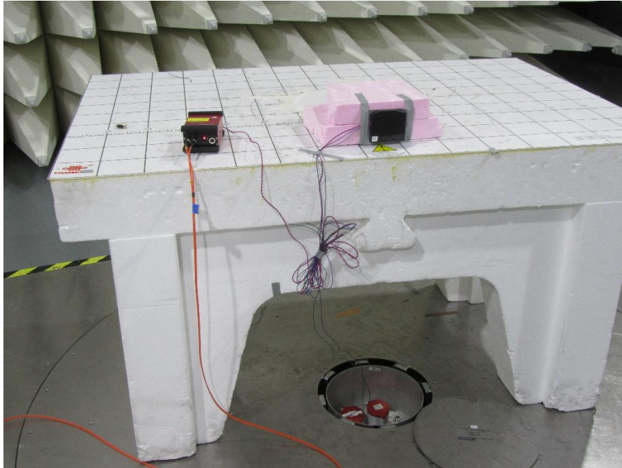
Radiated Emissions 9 kHz – 1 GHz
