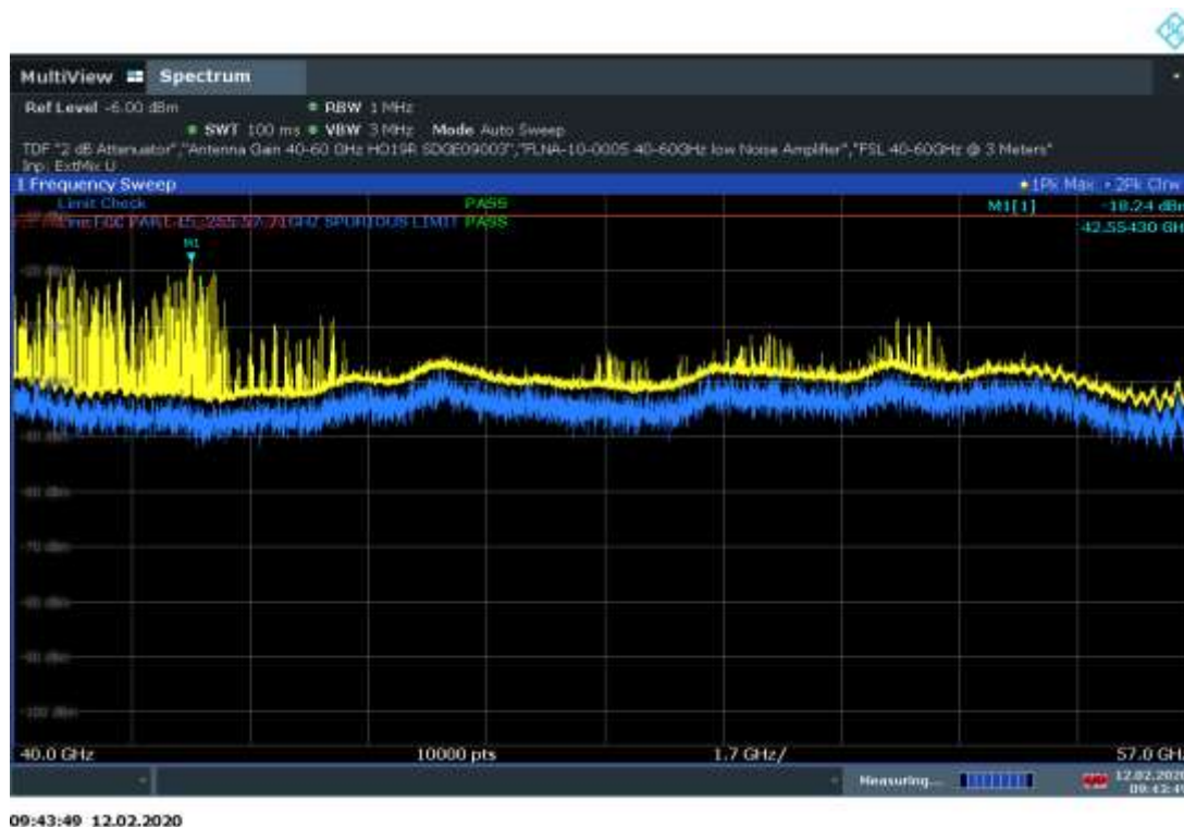
40GHz to 57GHz Plot (12 Transmitters)
