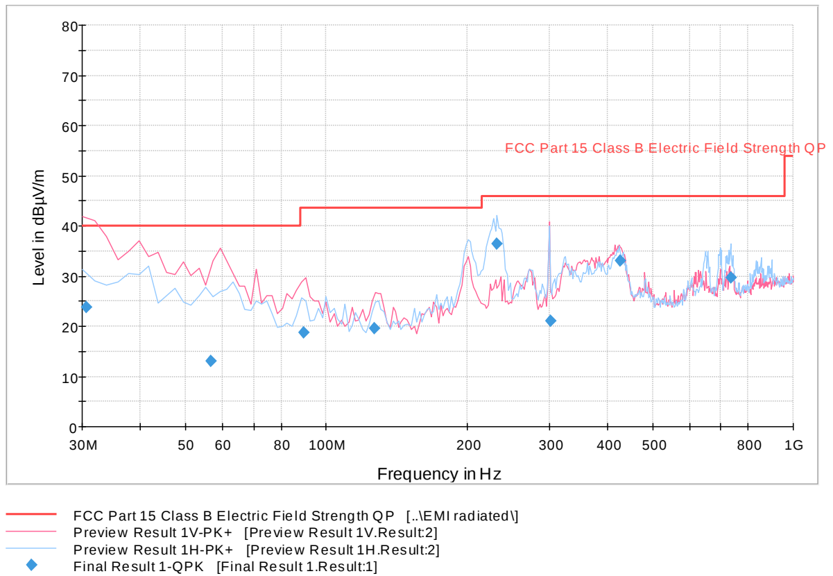
Continuous Rotation TUV 3m Radiated 30 to 1000MHz
