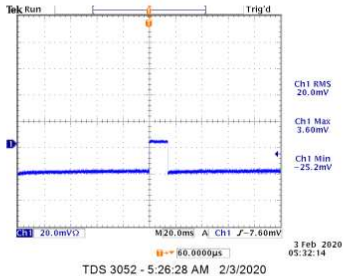
EUT (12 Transmitter) profile using a RF detector
