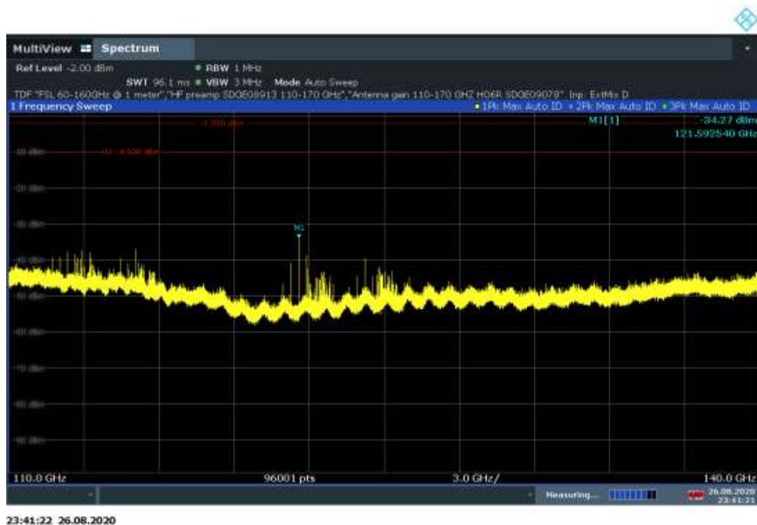
110GHz to 140GHz Plot (24 Transmitters)
