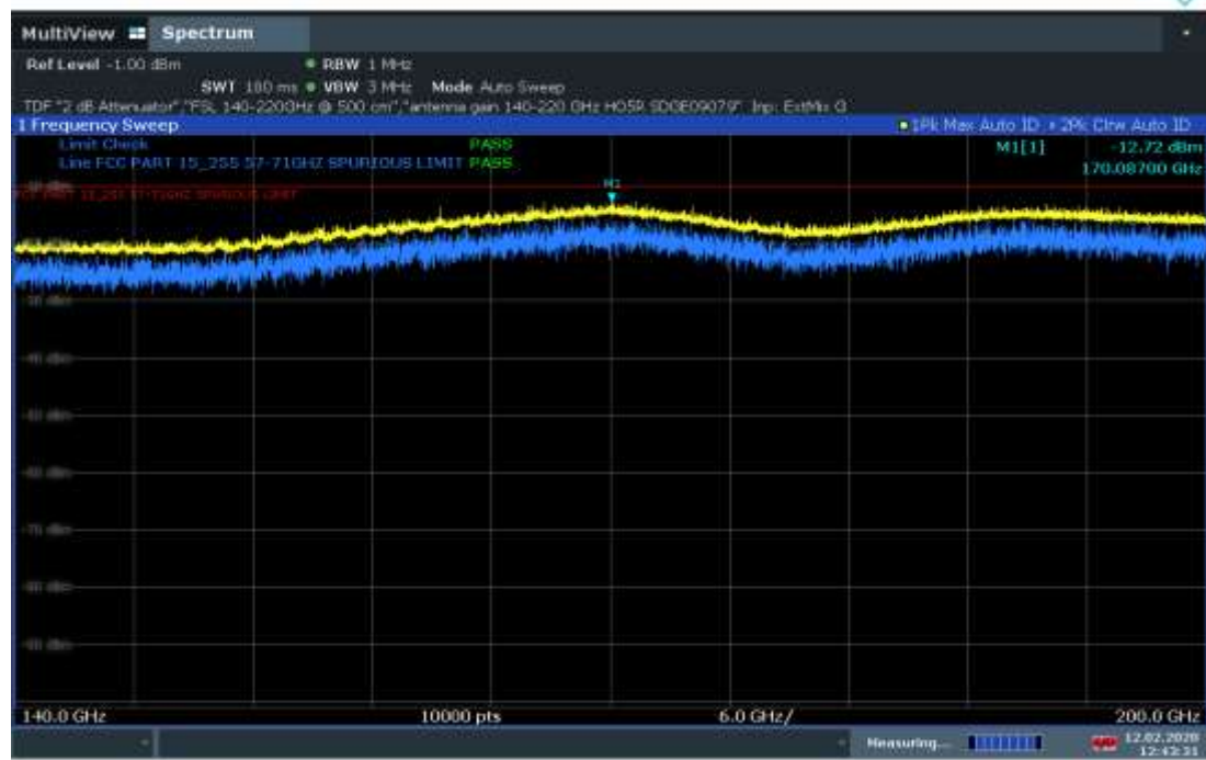
140GHz to 200GHz Plot (24 Transmitters)
