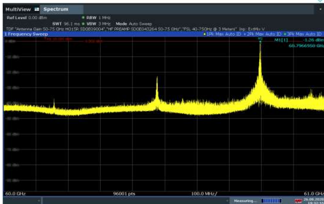
60GHz to 61GHz Plot (12 Transmitters)
