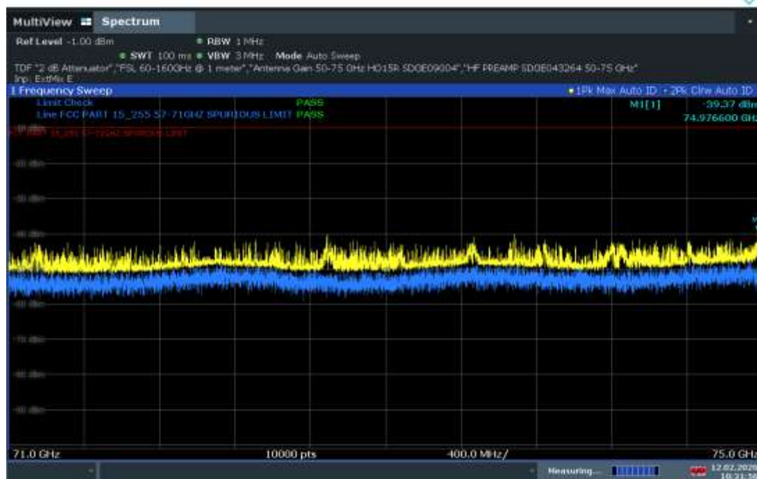
71GHz to 75GHz Plot (24 Transmitters)
