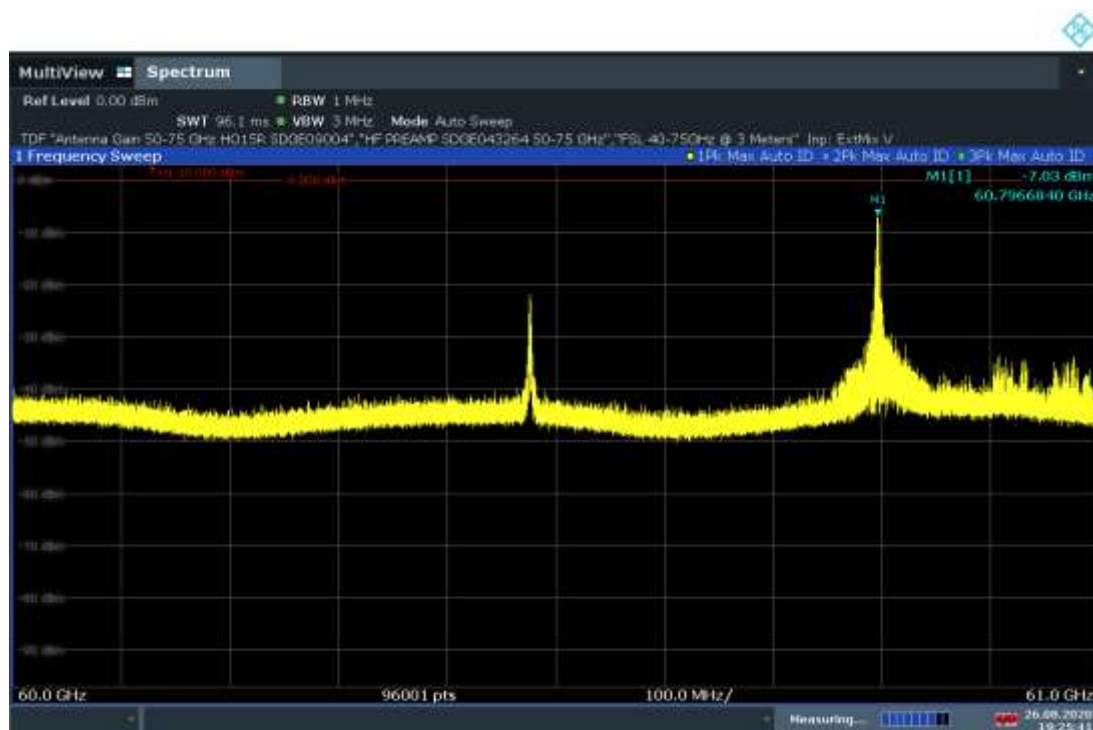
60GHz to 61GHz Plot (24 Transmitters)
