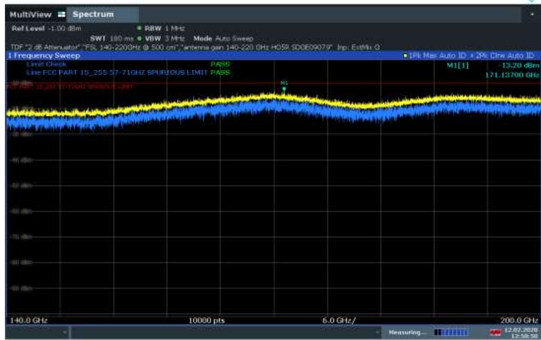
140GHz to 200GHz Plot (12 Transmitters)
