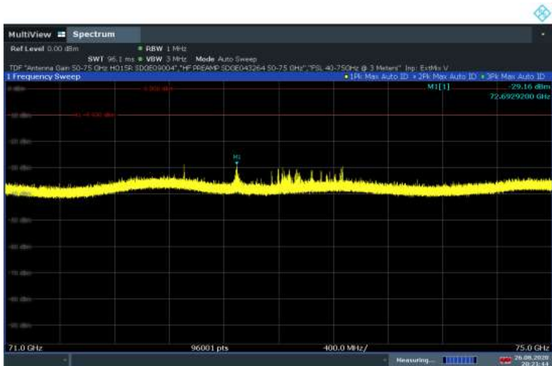
71GHz to 75GHz Plot (24 Transmitters)
