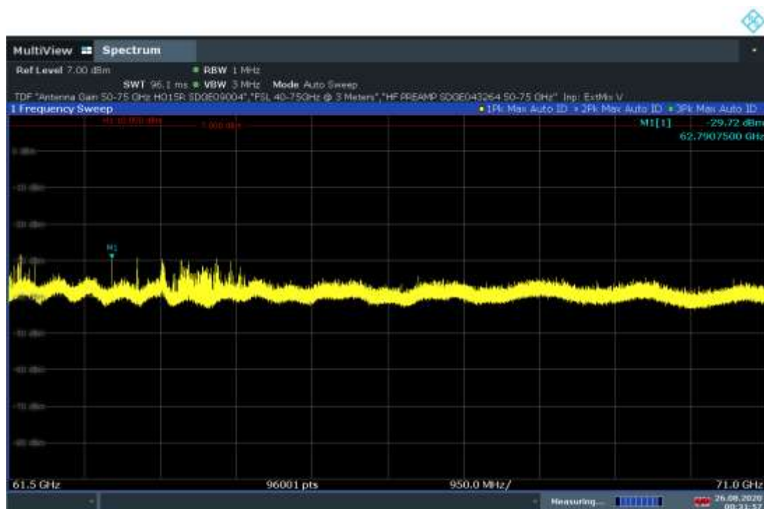
61GHz to 71GHz Plot (24 Transmitters)
