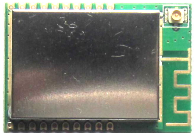
working with outside antenna
