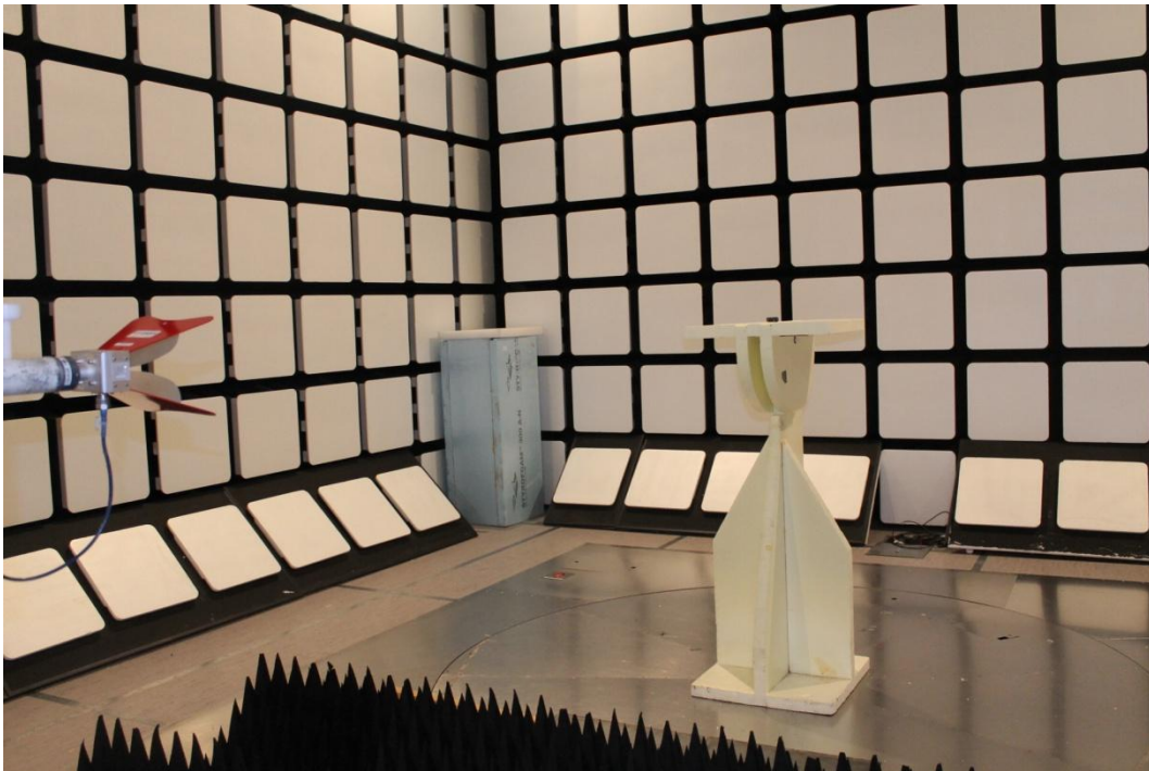
Photograph 4. Radiated emission setup (1-18 GHz).
