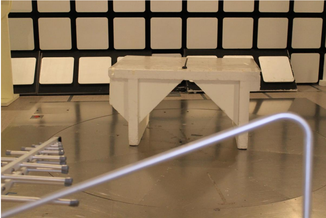
Photograph 3. Radiated emission setup (30-1000 MHz).
