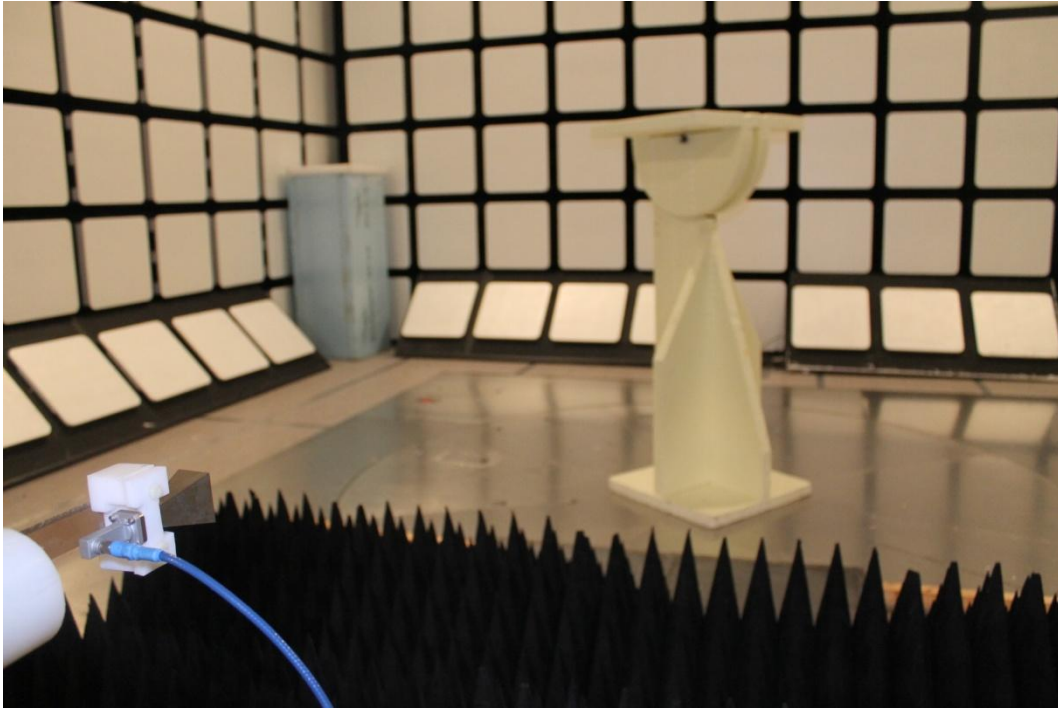
Photograph 5. Radiated emission setup (18-26.5 GHz).
