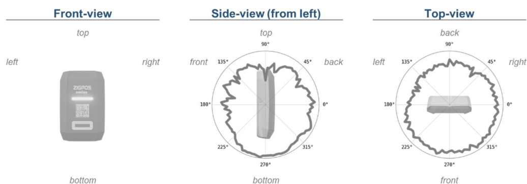
Figure 5 - Radio characteristics for 8 GHz UWB from front, side and top view
