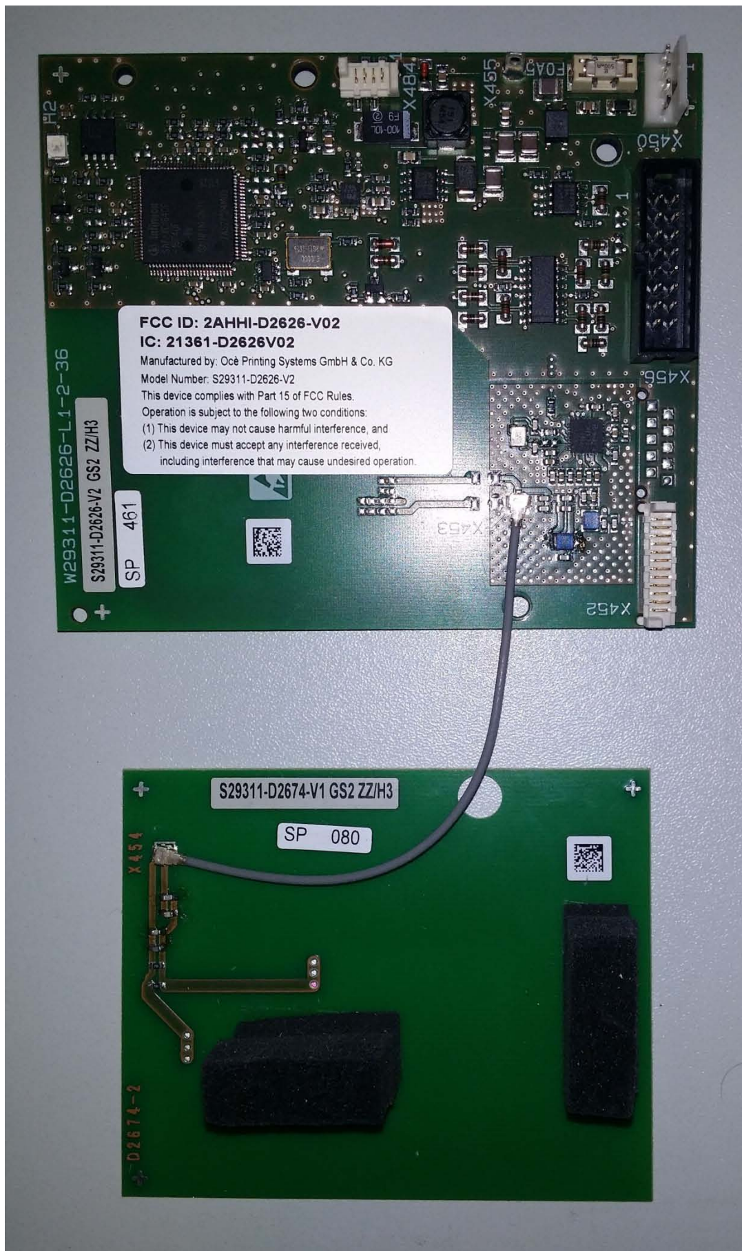
Figure 2: front side of S29311-D2626-V02 with PCB Antenna S29311-D2674-V1
