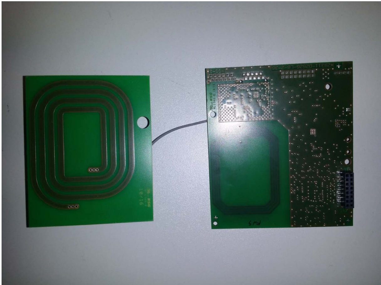
Figure 4: Rear side of S29311-D2626-V02 with PCB Antenna S29311-D2674-V1
