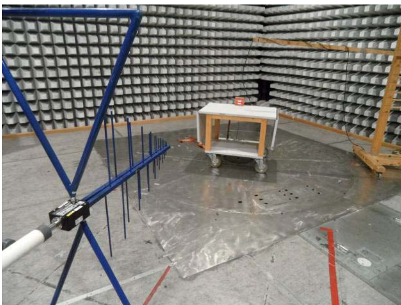
Figure 2: test setup for Radiated disturbances 30 MHz to 1000 MHz
