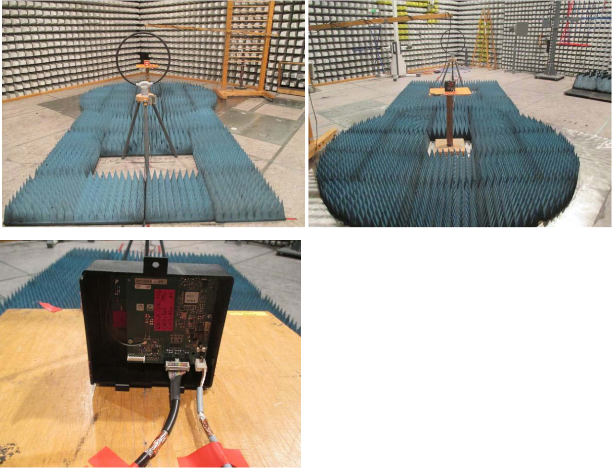
Figure 3: test setup for Radiated disturbances 9 kHz to 30 MHz
