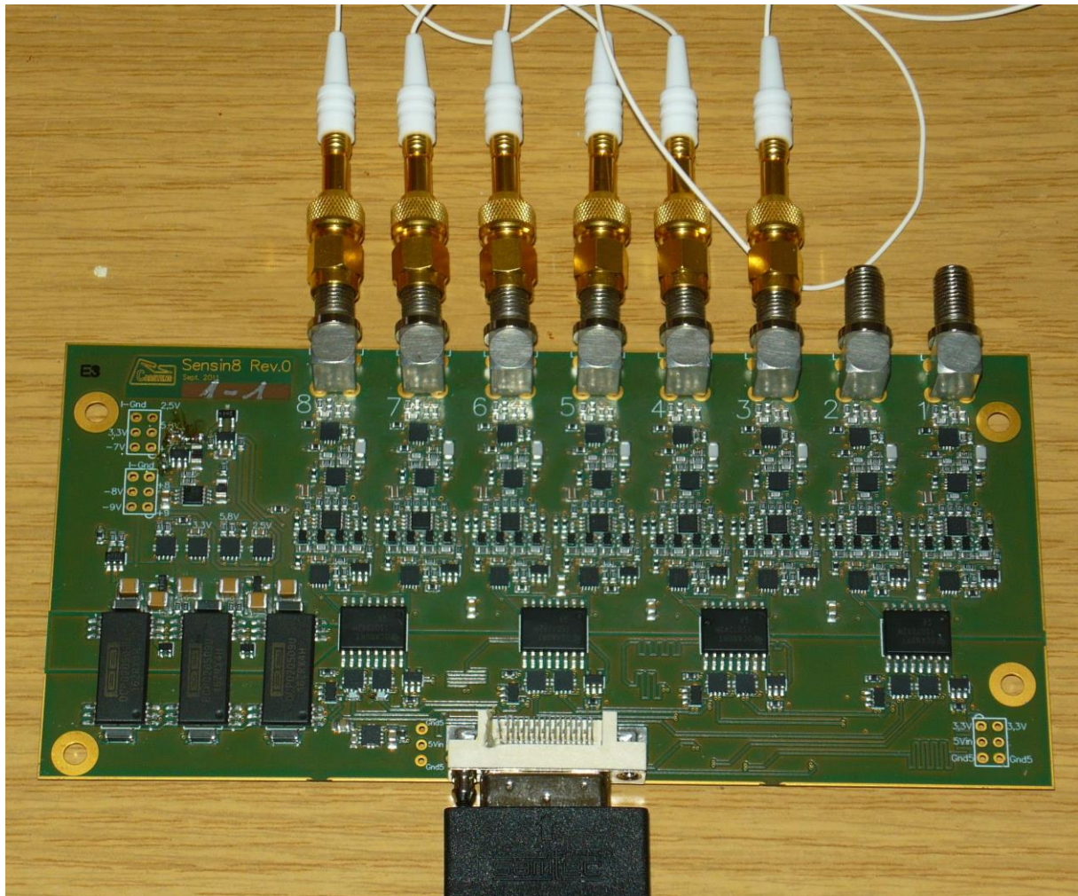
Figure 9 Sensin Board
