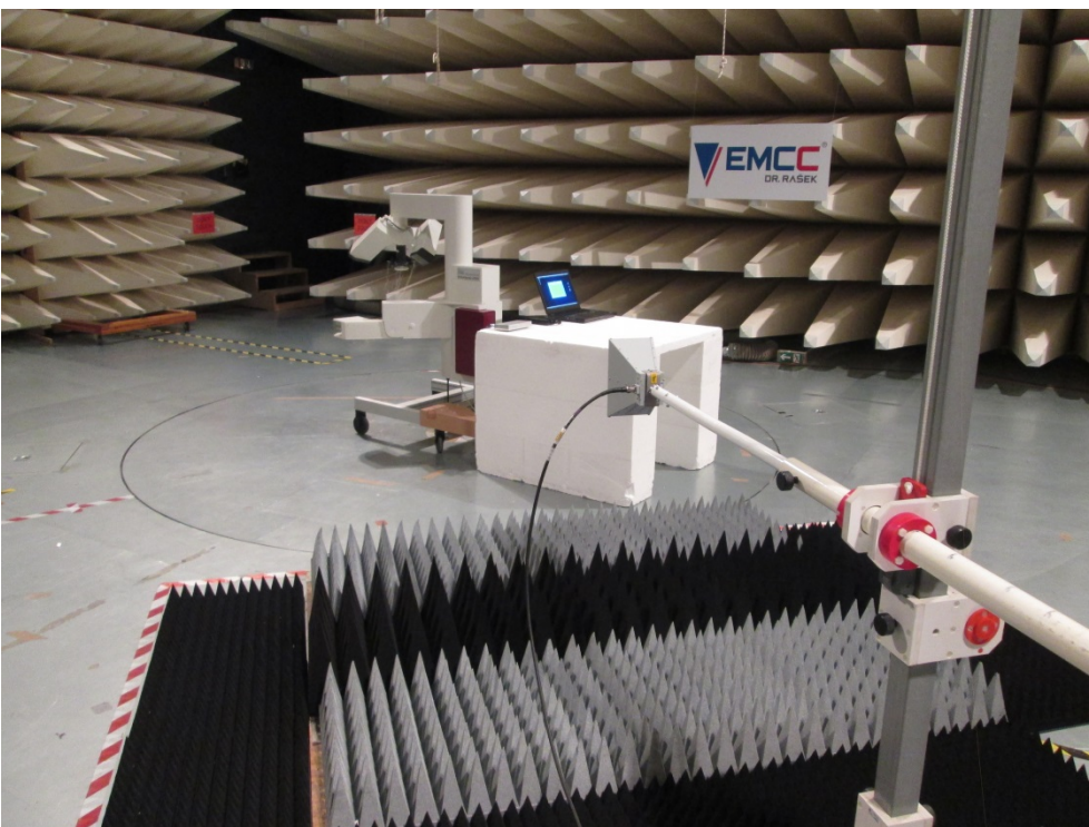
Photo A1-6: Radiated emissions measurement at 3 m distance, 1 GHz – 5 GHz
