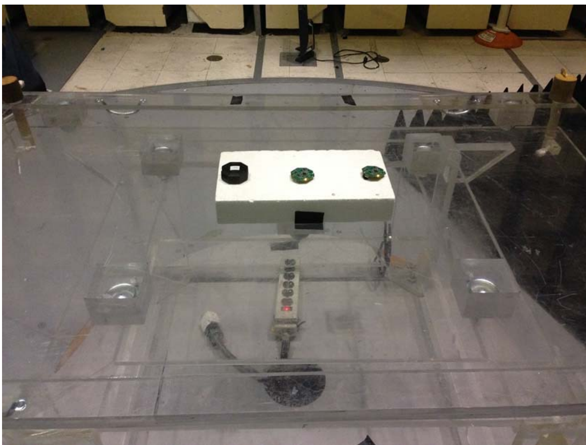
Radiated Emissions up to 18 GHz, Front
