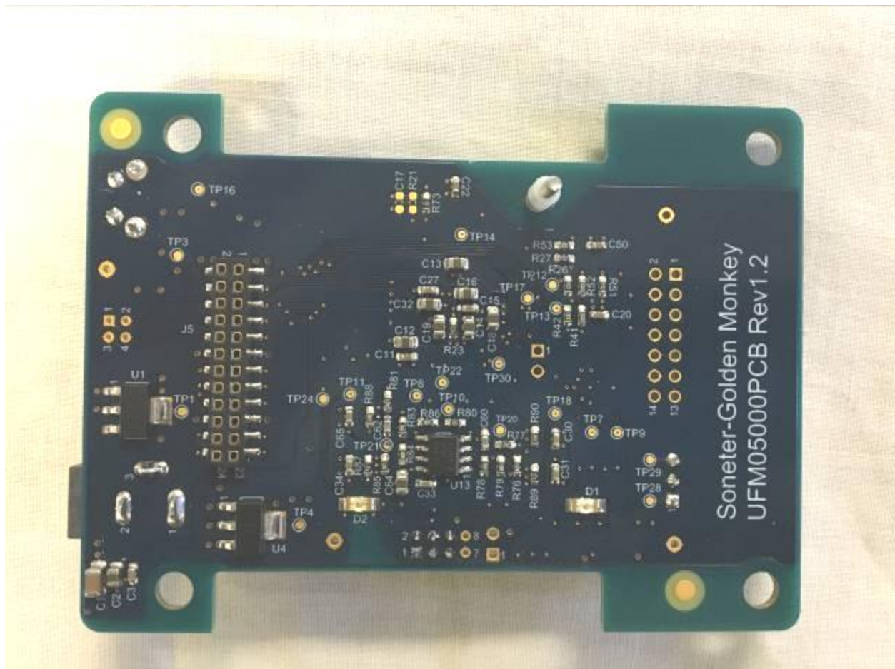
Figure 9. Main PCB (Bottom View)
