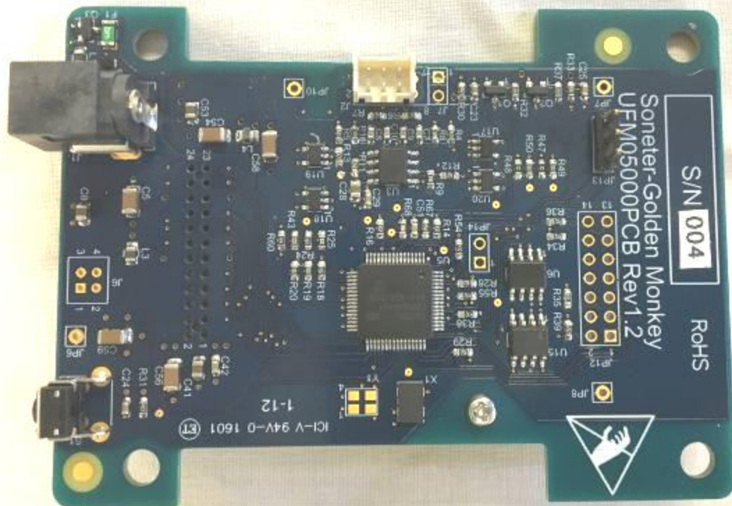
Figure 8. Main PCB (Top View)
