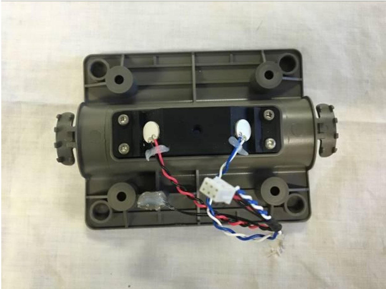
Figure 2. Bottom Cover (Internal View)
