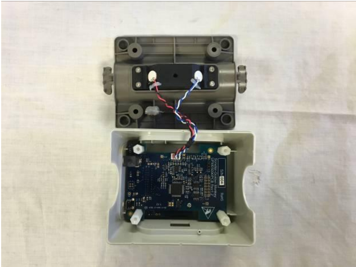
Figure 1. Bottom Cover Removed
