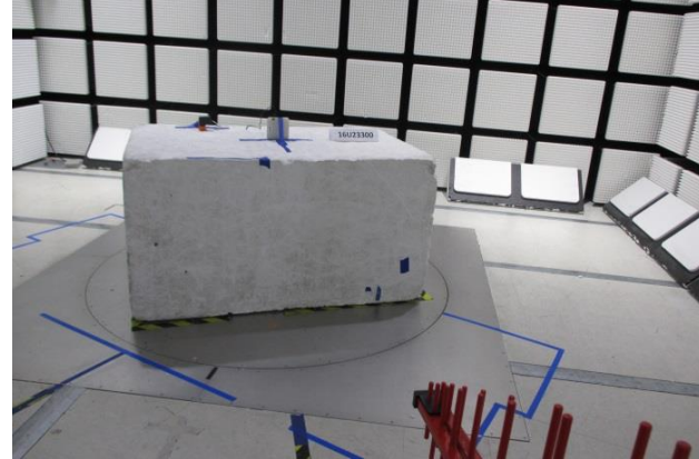
RADIATED FRONT PHOTO (ABOVE 1 GHz)
