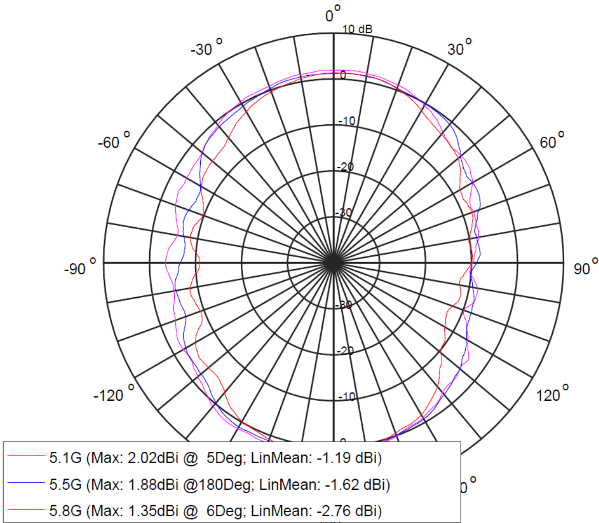
SMM EXT C1 ASK ANT1 YZ 5GHz Band
