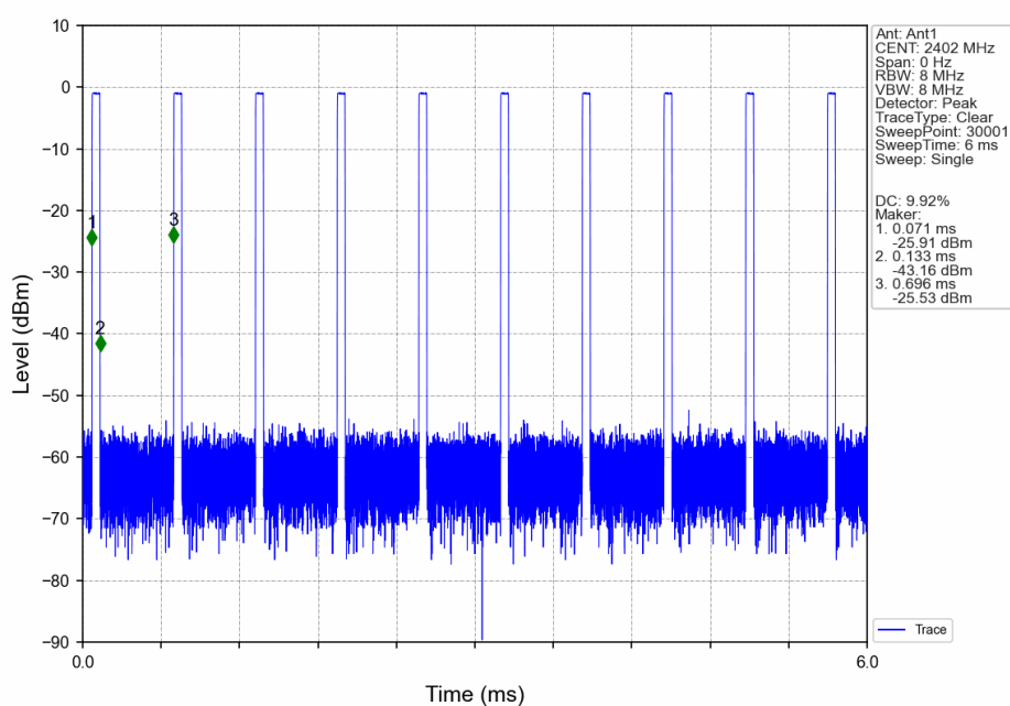
GFSK-2M_LCH_2402MHz_Ant1_NTNV
