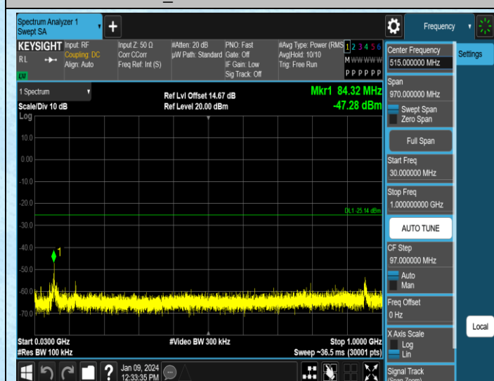
BLE_2M-Ant1-2402-30-1000
