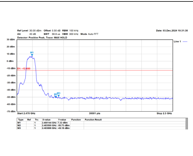
8DPSK(3DH5) (Band Edge) / 2480 MHz
