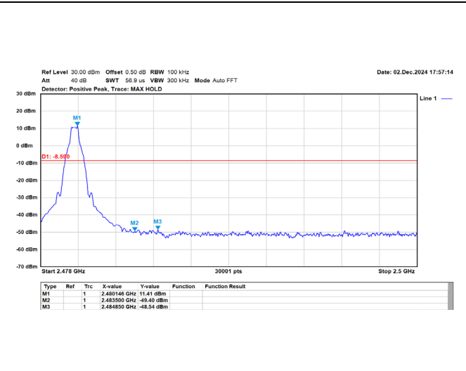
8DPSK(3DH5) (Band Edge) / 2480 MHz
