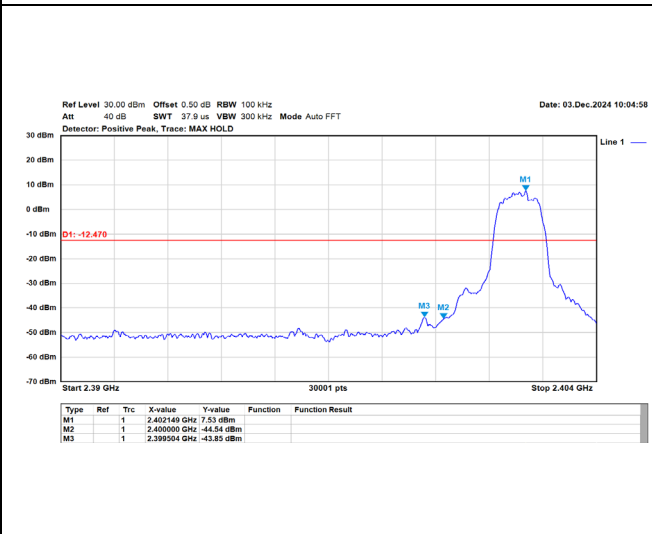
8DPSK(3DH5) (Band Edge) / 2402 MHz
