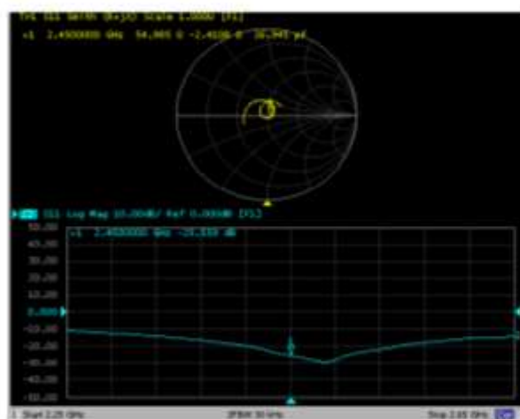
2450MHz Head
