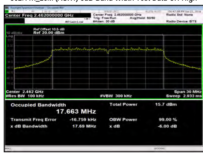
802.11n_20M (AUX1) 6dB Band Width Test Data CH-High
