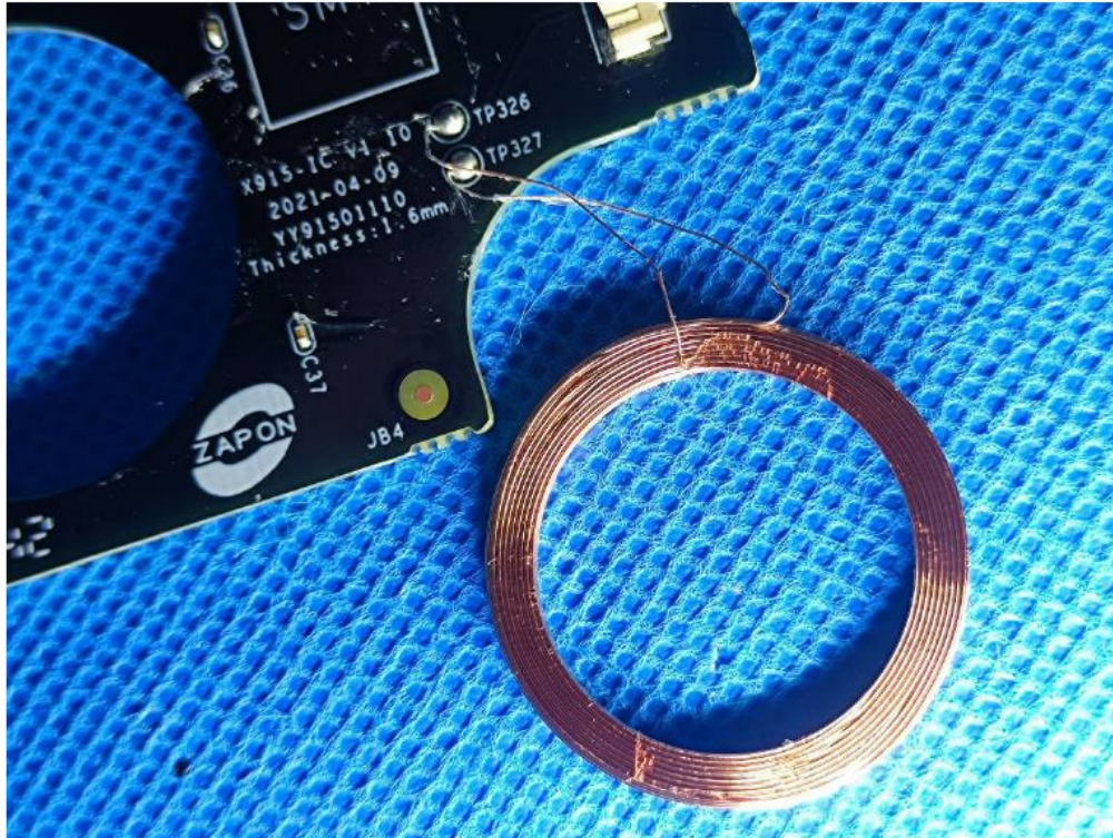
125kHz Antenna
