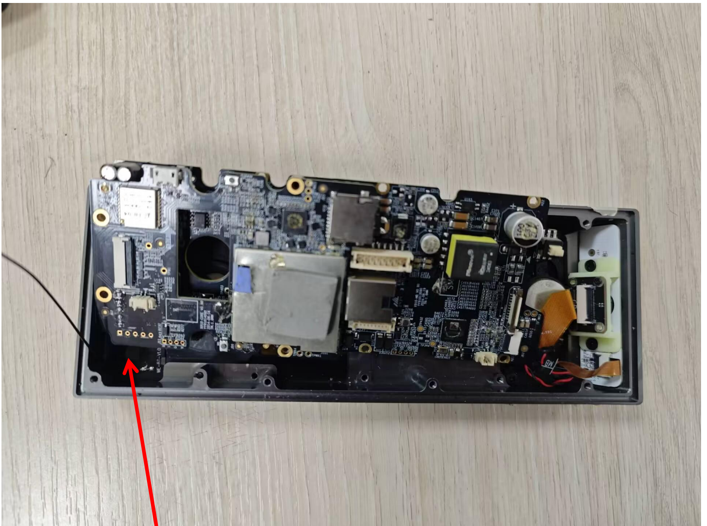
BT Antenna
