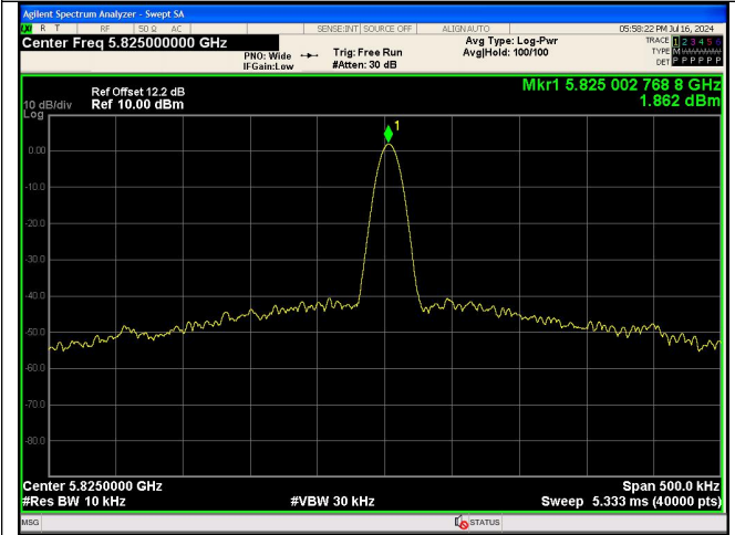
NT/NV_Antenna 0 IEEE 802.11ac_Channel 165_20MHz
