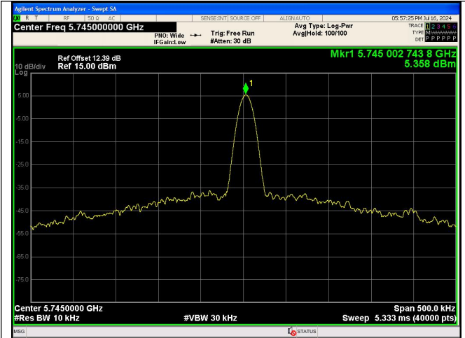
NT/NV_Antenna 0 IEEE 802.11ac_Channel 149_20MHz
