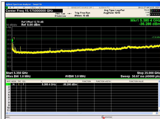
Spurious Emission:5350~25000.0 MHz IEEE 802.11ac_Channel 40_20MHz_Antenna 0
