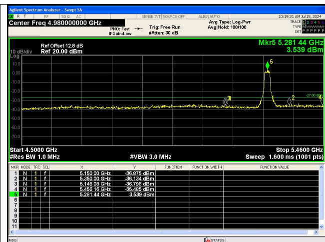
Out Of Band Emission IEEE 802.11ac_Channel 56_20MHz_Antenna 0
