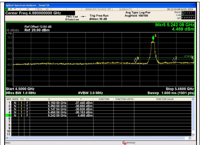
Out Of Band Emission IEEE 802.11ac_Channel 48_20MHz_Antenna 0
