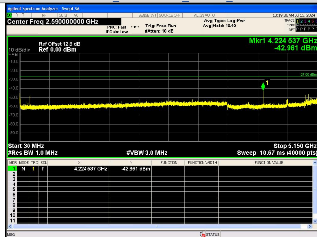
Spurious Emission:30.0~5150 MHz IEEE 802.11ac_Channel 56_20MHz_Antenna 0
