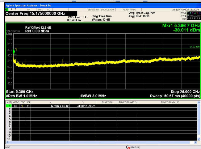
Spurious Emission:5350~25000.0 MHz IEEE 802.11ac_Channel 56_20MHz_Antenna 0
