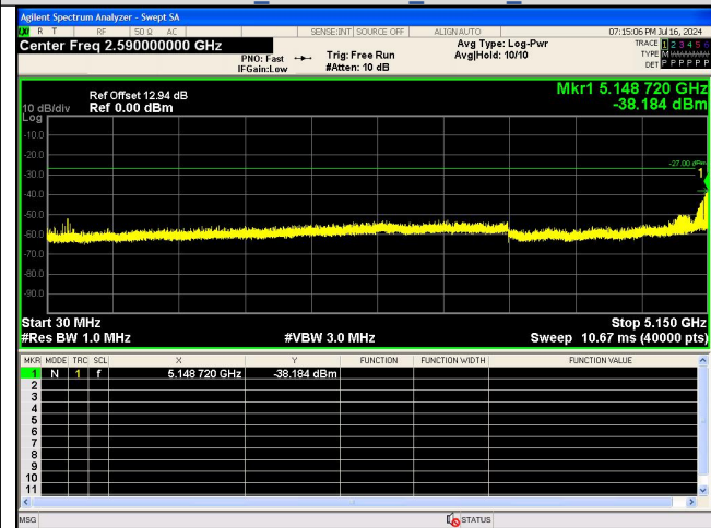
Spurious Emission:30.0~5150 MHz IEEE 802.11ac_Channel 64_20MHz_Antenna 0
