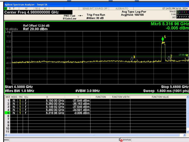
Out Of Band Emission IEEE 802.11ac_Channel 64_20MHz_Antenna 0
