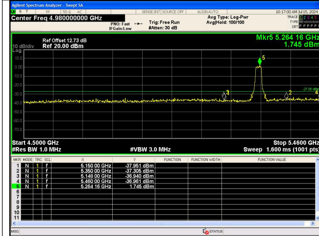
Out Of Band Emission IEEE 802.11ac_Channel 52_20MHz_Antenna 0
