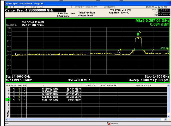
Out Of Band Emission IEEE 802.11n_Channel 54_40MHz_Antenna 0
