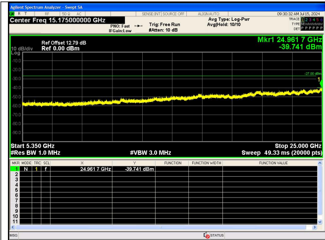
Spurious Emission:5350~25000.0 MHz IEEE 802.11n_Channel 38_40MHz_Antenna 0
