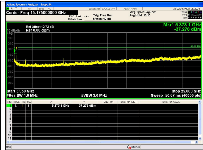
Spurious Emission:5350~25000.0 MHz IEEE 802.11n_Channel 52_20MHz_Antenna 0
