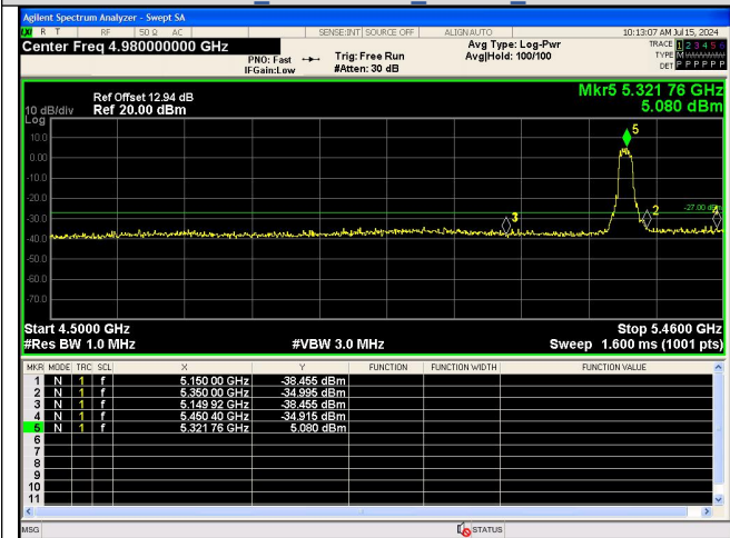
Out Of Band Emission IEEE 802.11n_Channel 64_20MHz_Antenna 0
