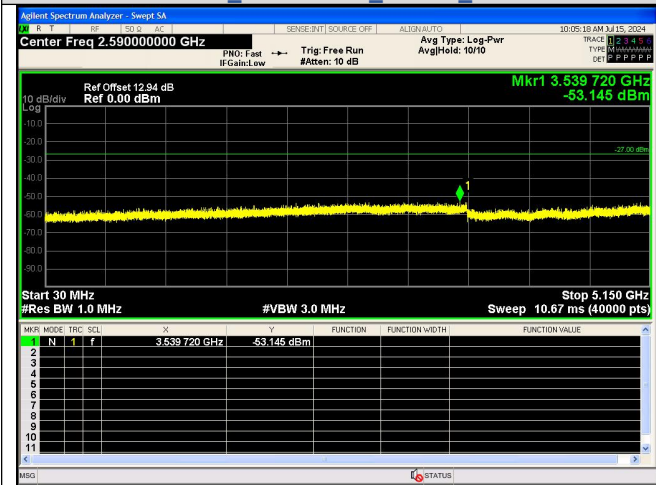
Spurious Emission:30.0~5150 MHz IEEE 802.11a_Channel 64_20MHz_Antenna 0
