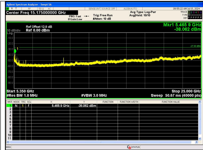
Spurious Emission:5350~25000.0 MHz IEEE 802.11a_Channel 56_20MHz_Antenna 0
