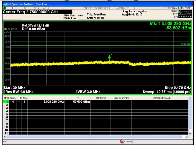
Spurious Emission:30.0~5470 MHz IEEE 802.11a_Channel 100_20MHz_Antenna 0
