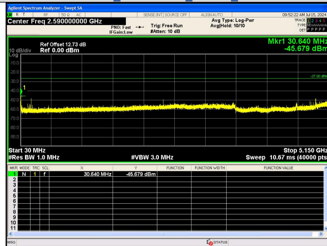
Spurious Emission:30.0~5150 MHz IEEE 802.11a_Channel 52_20MHz_Antenna 0
