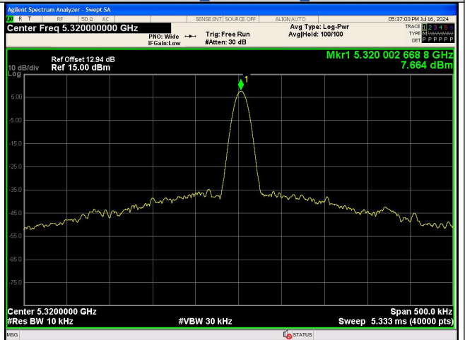
NT/NV_Antenna 0 IEEE 802.11a_Channel 64_20MHz
