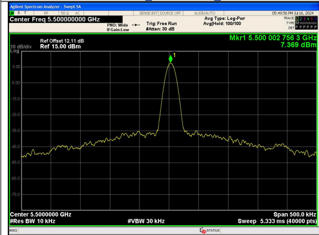
NT/NV_Antenna 0 IEEE 802.11ac_Channel 100_20MHz
