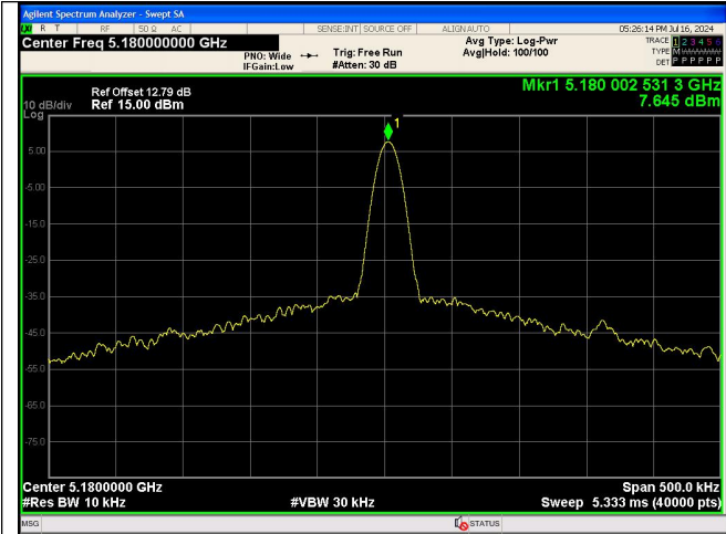
NT/NV_Antenna 0 IEEE 802.11a_Channel 36_20MHz
