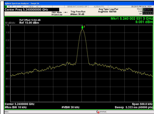
NT/NV_Antenna 0 IEEE 802.11n_Channel 48_20MHz
