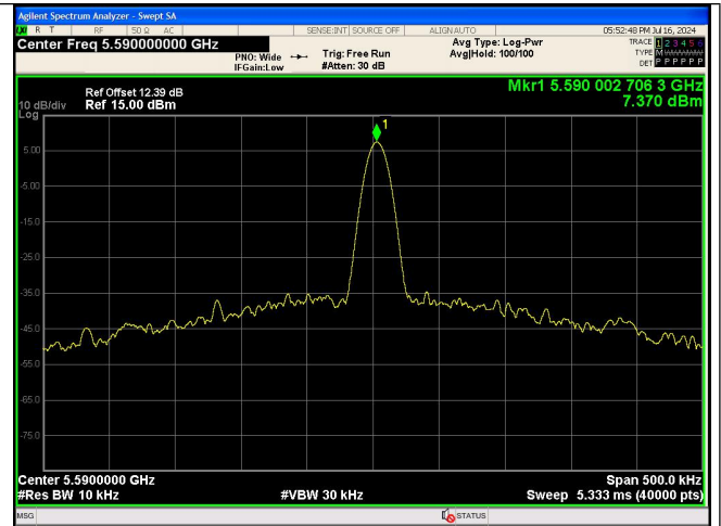
NT/NV_Antenna 0 IEEE 802.11n_Channel 118_40MHz
