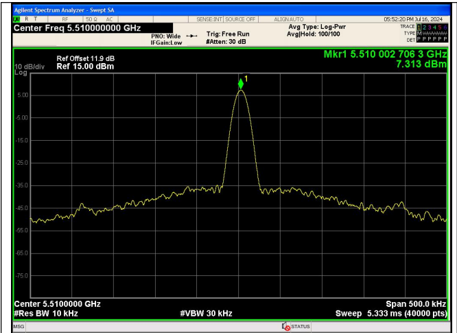
NT/NV_Antenna 0 IEEE 802.11n_Channel 102_40MHz
