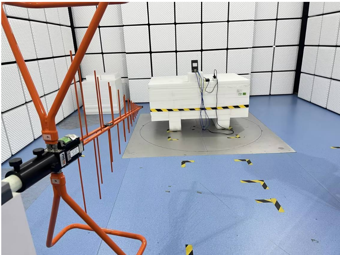
RE-Back View(30MHz~1GHz)(POE)
