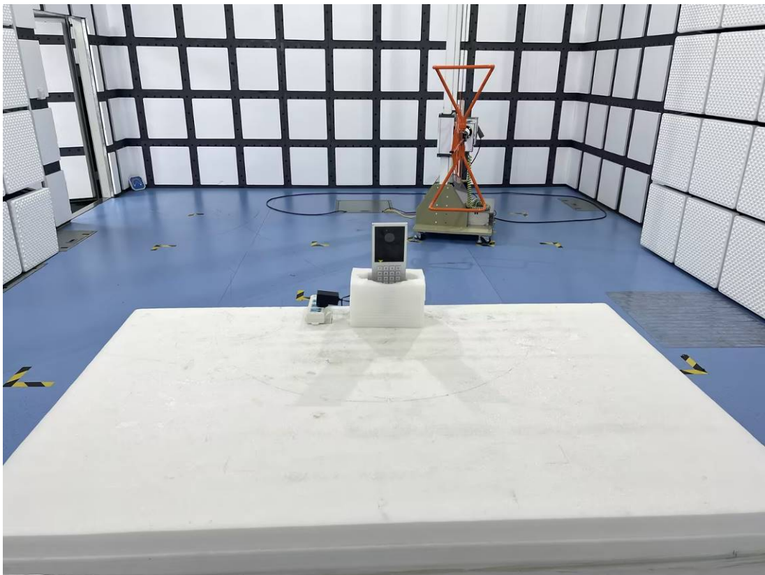
RE-Front View(30MHz~1GHz)(Adapter)
